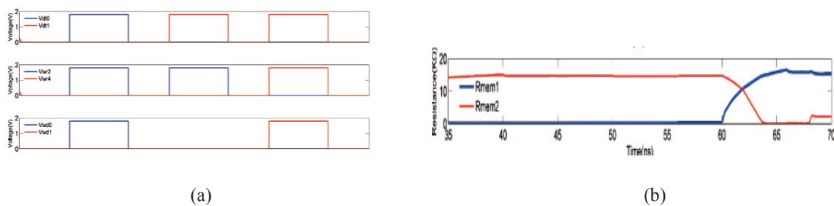
Figure 4. (a) Timing diagram of input pulses during write operation. (b) Change of resistance of the two memristors of cell20 during write operation.
