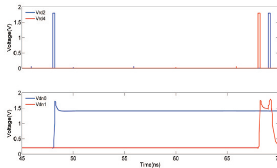
Figure 5. Proof of non-volatility of the memristor SRAM cell.
