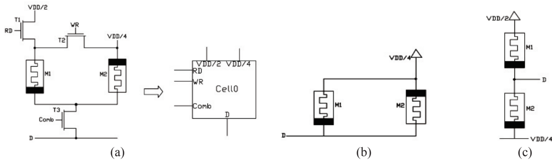
Figure 3. (a) Three transistor-two memristor SRAM cell (b) Circuit when rd=0, wr=1, and comb =1. (c) Circuit when rd=1, wr=0, and Comb=1.
