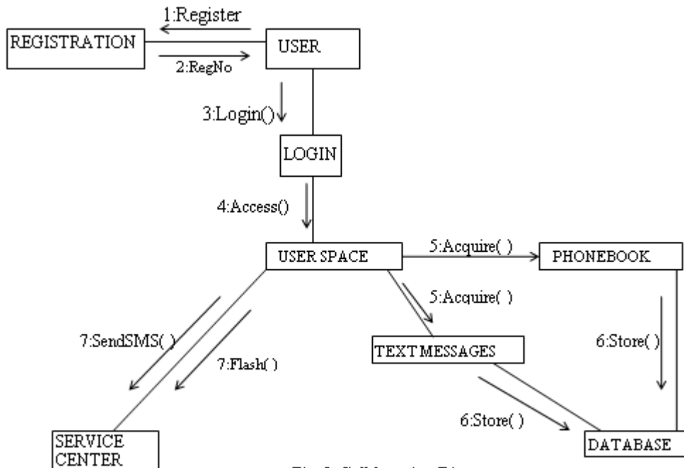
Fig. 9: Collaboration Diagram
