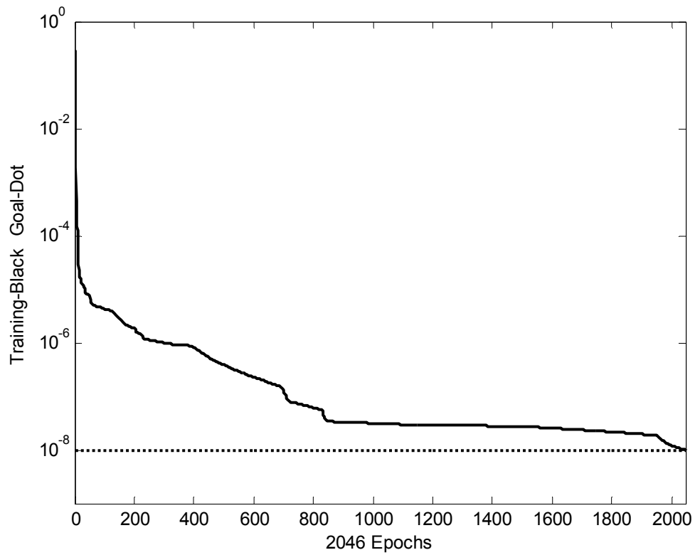
Figure 7: Error with epochs during training of ANN Modeling for inrush current
