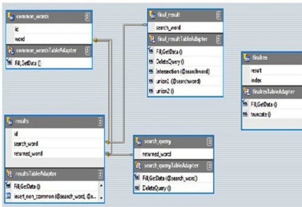
Figure 2: The database that is used in our project
