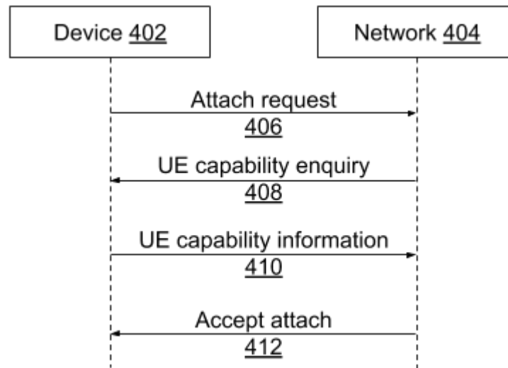
Fig. 4: Device-network messaging to communicate UE capability
