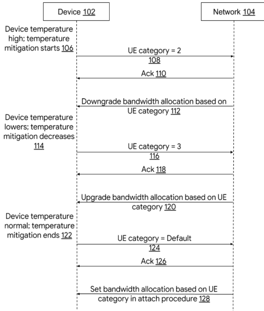
Fig. 1: Temperature mitigation using UE category to set downlink bandwidth allocation
