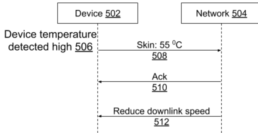
Fig. 5: Device-network messaging to mitigate temperature in a network-centric approach
