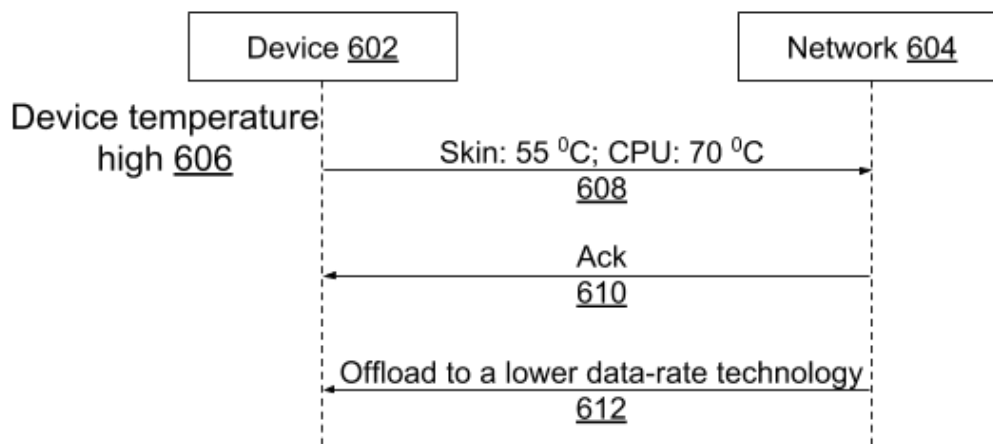
Fig. 6: Device-network messaging to mitigate temperature in a network-centric approach
