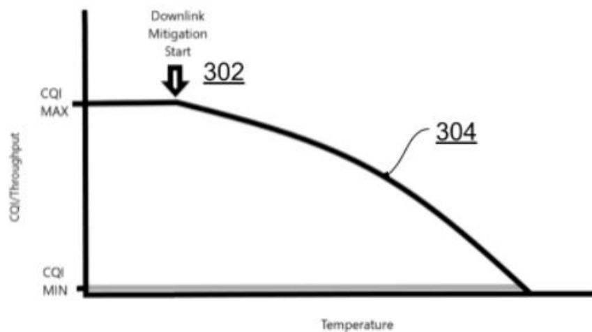
Fig. 3: Throughput against temperature
