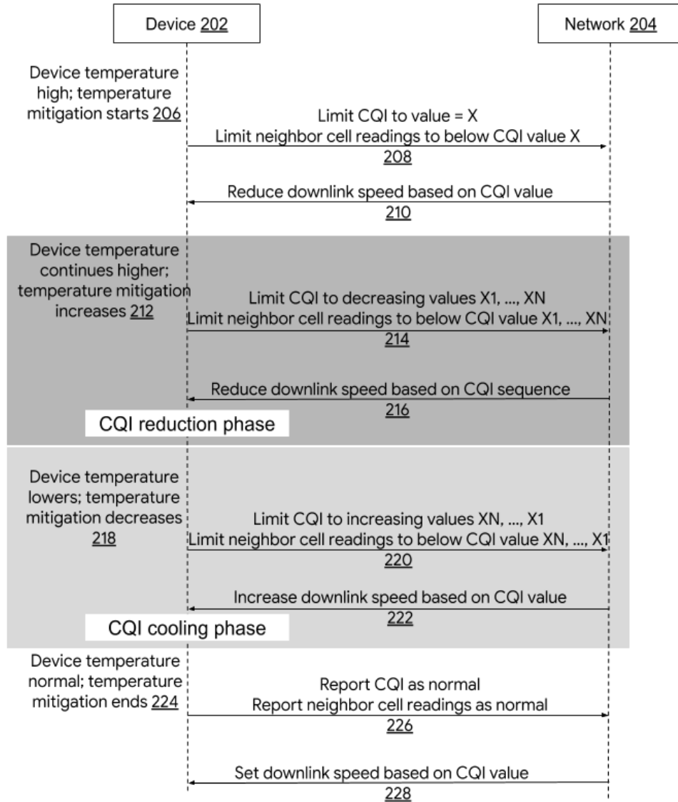
Fig. 2: Temperature mitigation using CQI to set downlink throughput
