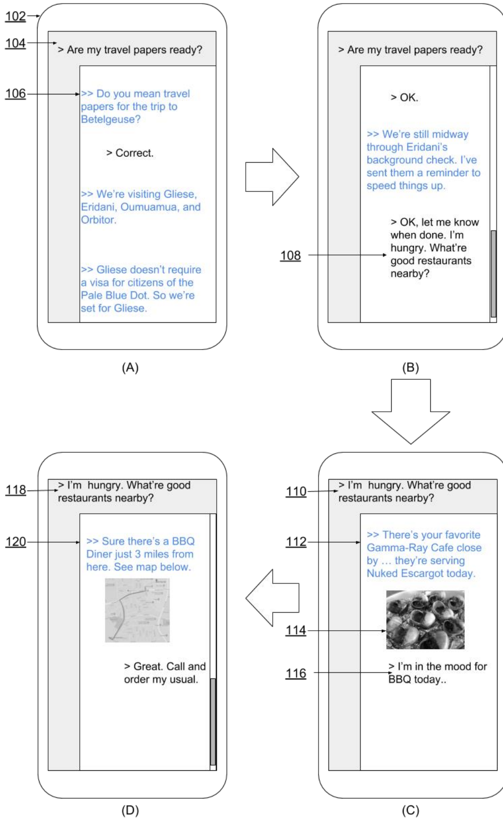
Fig. 1: Conversational hierarchy for interaction with virtual assistant
