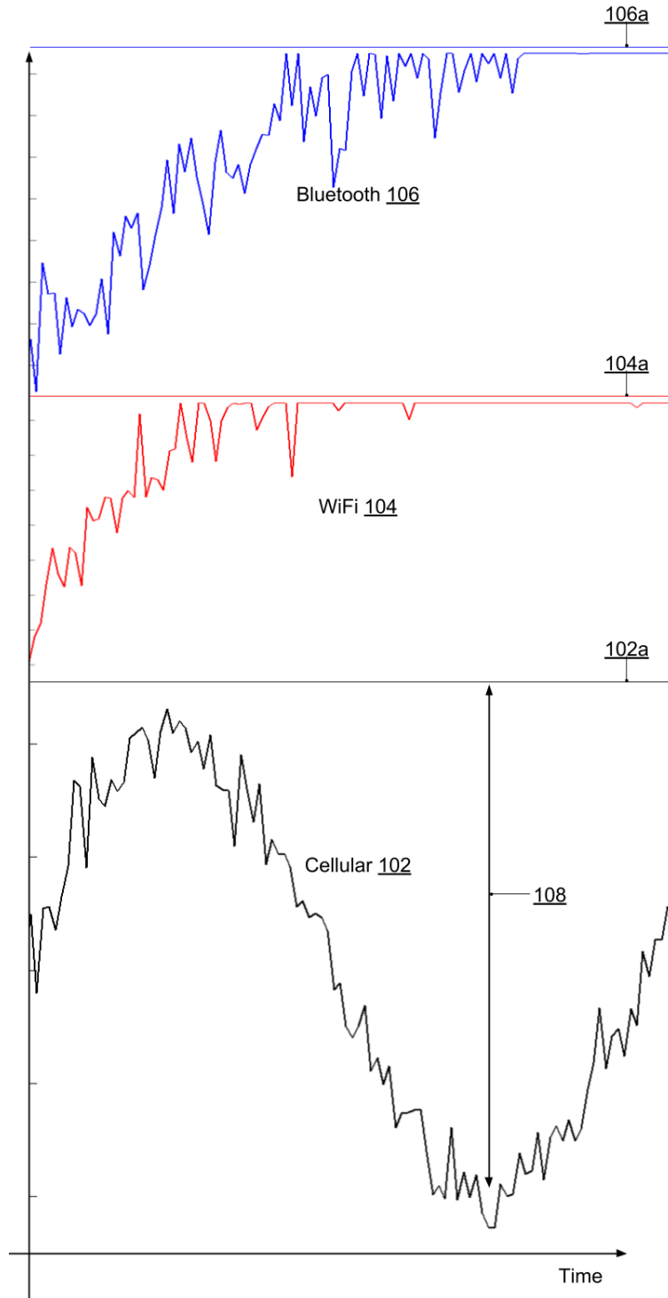
Fig. 1: A radio that does not take advantage of low actual transmit powers of another radio
