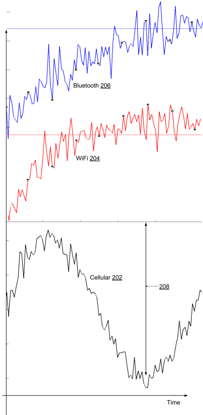
Fig. 2: Computing maximum power of a radio based on actual transmit power of other radios
