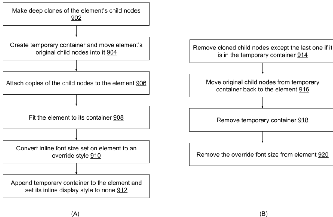
Fig. 9: (A) Text-fitting via truncation of text, and (B) its reversal, per the second technique
