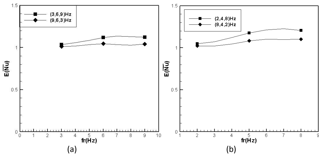
Figure.10 The variation of the heat transfer enhancement factor for various continuous frequencies (a) q'' = 85 \text{ W/m}^2 (b) q'' = 946.017 \text{ W/m}^2 .
