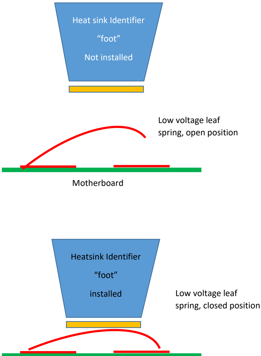
Figure 3 – shows how heatsink’s “one foot” depresses motherboard switch to close the circuit.
