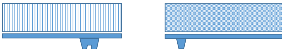
Figure 1 – A heatsink using method 1 which has two points of contact to motherboard’s mating leaf spring connector (“two feet”)
