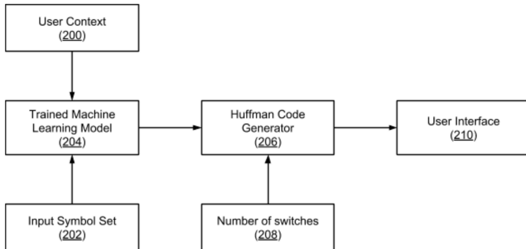
Fig. 2: Generating a Huffman tree for switch input using a trained machine learning model
