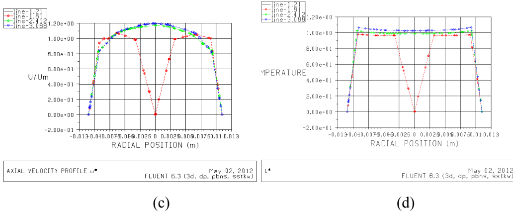
Fig. 5 (a) Dimensionless Axial Velocity vs Radial Position for FLTT (b) Dimensionless Temperature vs Radial Position for FLTT (c) Dimensionless Axial Velocity vs Radial Position for HLUTT (d) Dimensionless Temperature vs Radial Position for HLUTT
