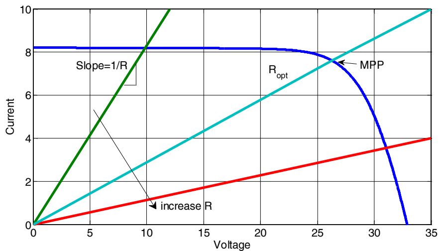
Fig.3. I-V curves of PV array and various resistive loads
