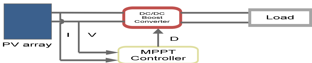
Fig.4. MPPT system
