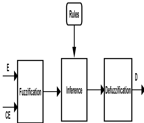
Fig.8. Fuzzy controller diagram
