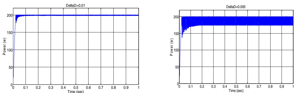
Fig.7. P&O MPPT for different \Delta D
