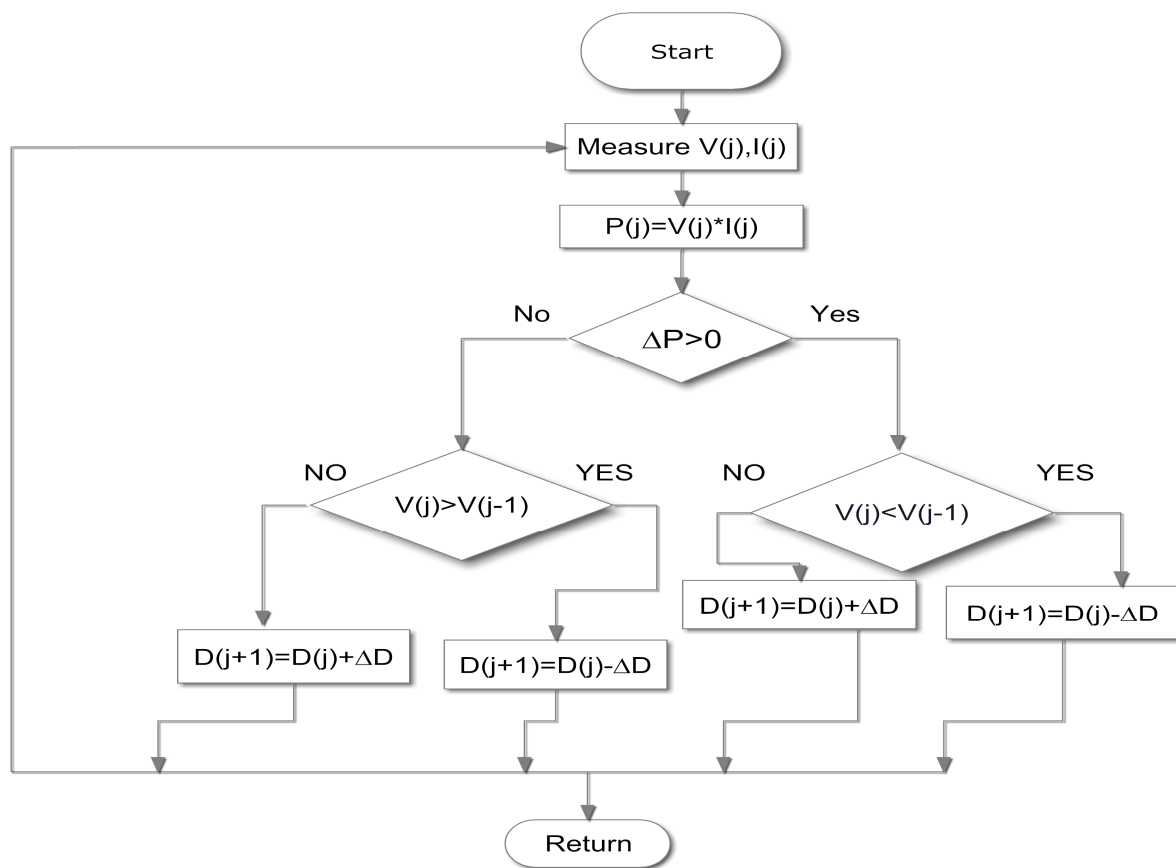
Fig.6. P&O flowchart
