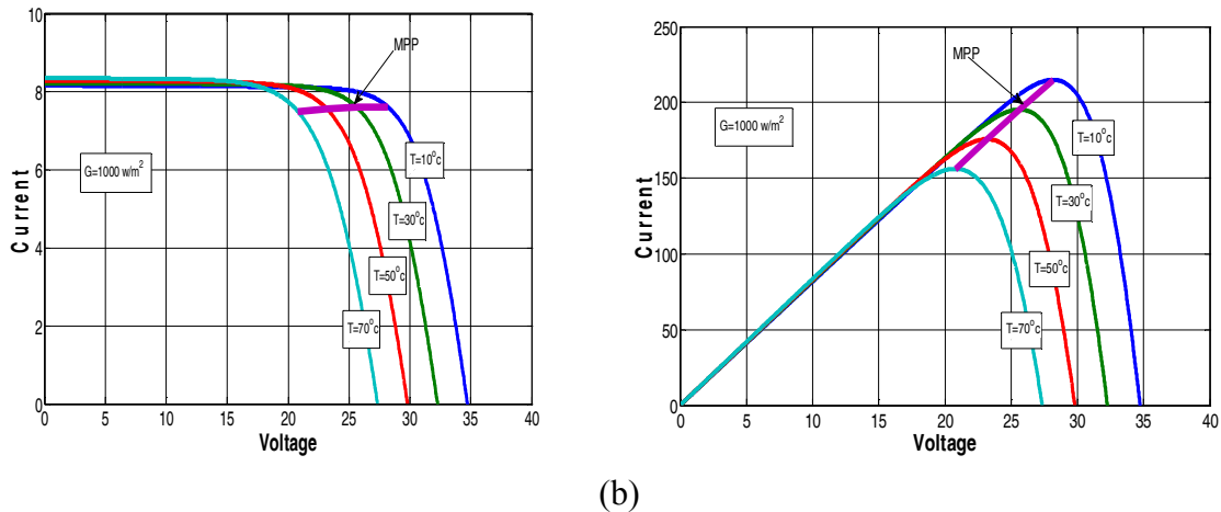
Fig.2. (a) V-I ,P-V Characteristics of PV module at constant temperature and varying insulations,(b) V-I ,P-V Characteristics of PV module at constant insulations and varying temperature.
