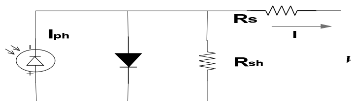
Fig.1. PV modeling
