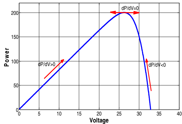
Fig.9.p-v curve at 1000 w/m2
