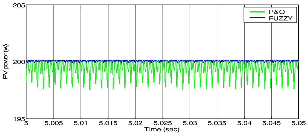
Fig13.Simulation result at constant temperature and insolation
