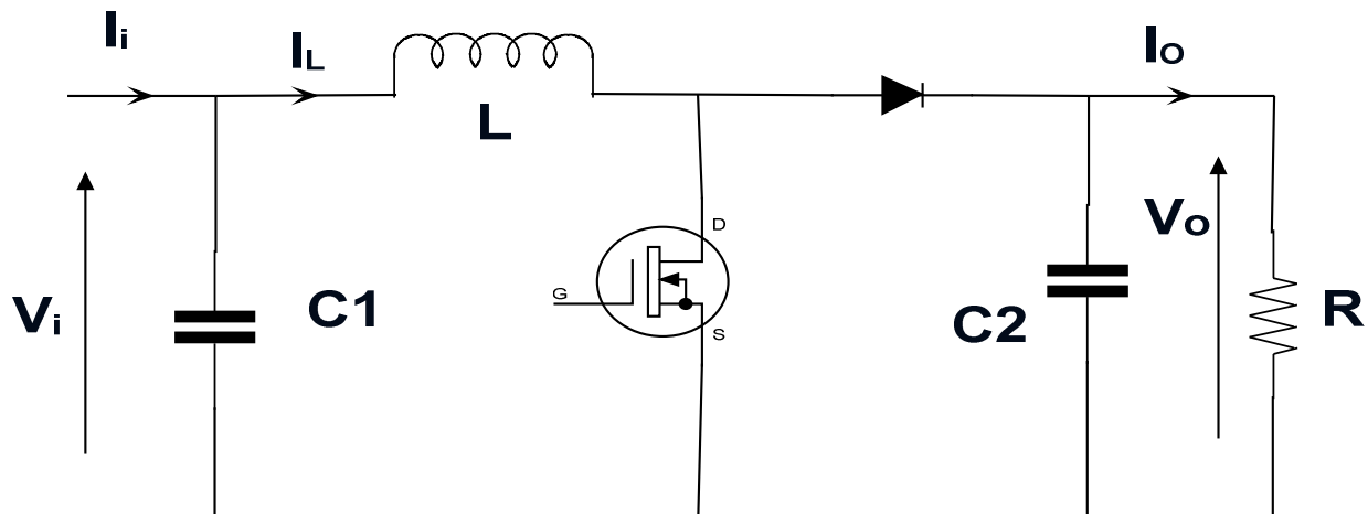
Fig.5. Boost converter Circuit diagram
