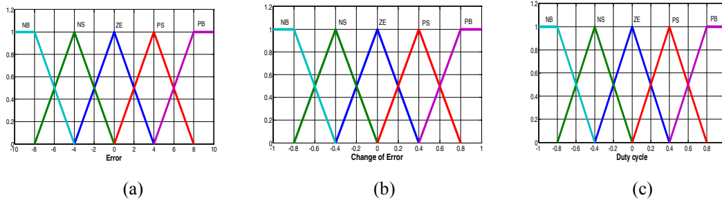
Fig.10. Membership function of E, CE and D
