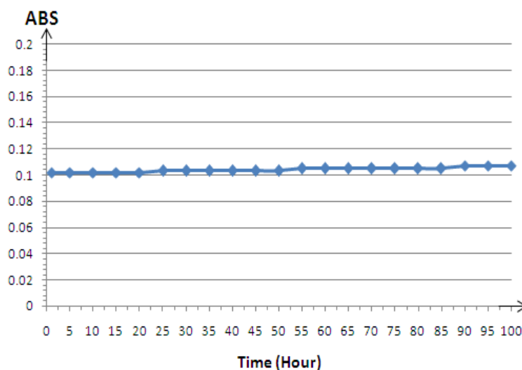
Figure(14): Absorbance change with time, where the concentration is equal to (1.5 \times 10^{-5}M) for each of metal ions solution and reagent solution in the same solution.
