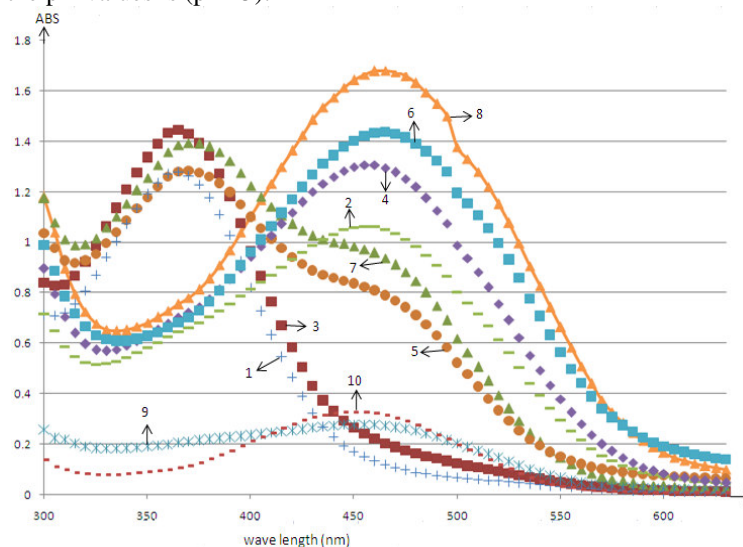
Figure(11): Change of absorption spectrum of the reagent solution by adding the metal ions solution, where the concentration is ( 9.6 \times 10^{-4} \text{M} ) for both of them at Selected pH values:
