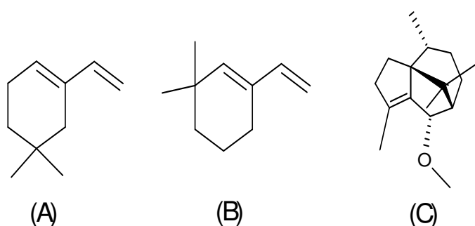
Figure 1: Isolated compounds from X. aethiopicica root bark extract [Yapi et al, 2012 ]: (A) 4,4-dimethyl-2-vinylcyclohexene (xylopiya A), (B) 3,3-dimethyl-1-vinylcyclohexene (xylopiya B), and (C) endo-5-methoxy-3-patchoulene (xylopiya C).
