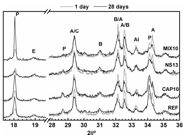
Fig. 3. X-ray diffractograms of cement pastes at 1 and 28 days.
