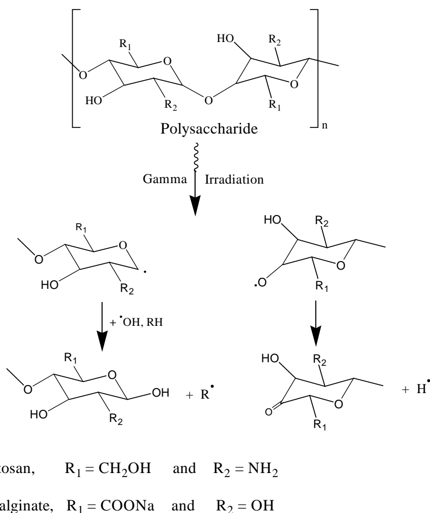
Scheme (1): Proposed mechanism of radiation induced degradation of chitosan and Na-alginate
