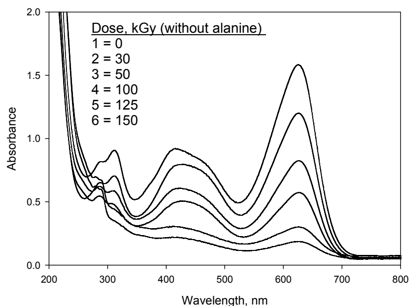
Fig. (1): The absorption spectra of (BTB-MO)/PVA films unirradiated and irradiated to different absorbed doses.
