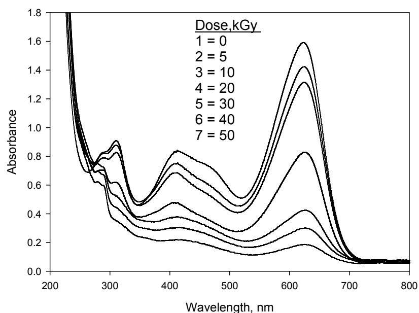
Fig. (2): The absorption spectra of (BTB-MO)/PVA films unirradiated and irradiated to different absorbed doses. [Alanine] = 66.66 phr
