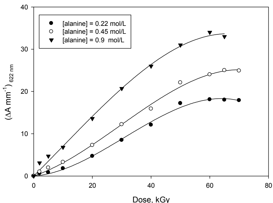
Fig. (3): Change of absorbance at 622 nm as a function of absorbed dose of (BTB-MO)/PVA films with different concentrations of alanine.
