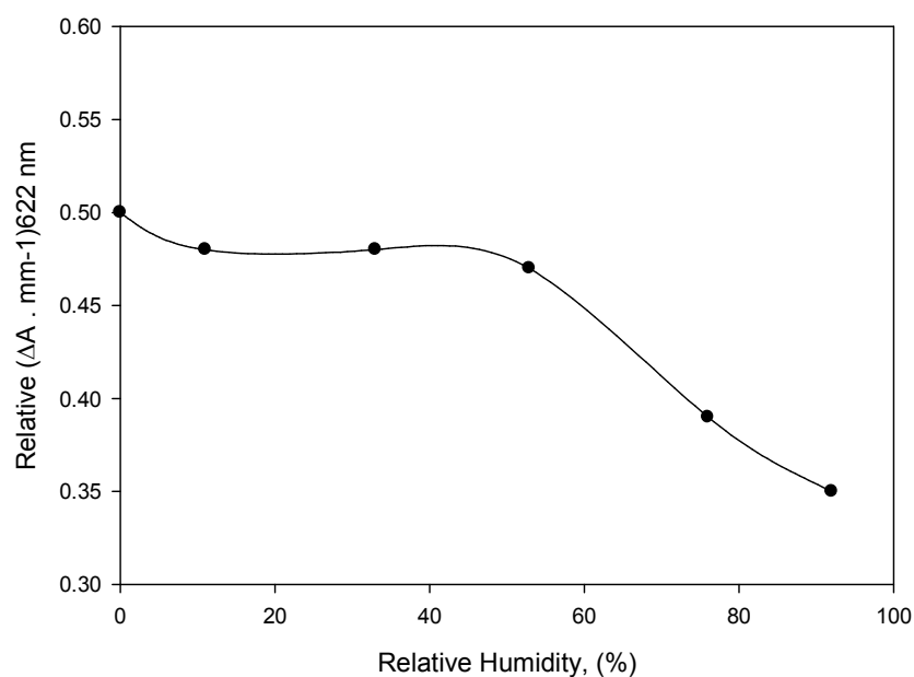
Fig. (5): Variation of response of (BTB-MO)/PVA films (at 622 nm) as a function of relative humidity during irradiation, where response in \Delta A \cdot \text{mm}^{-1} at 30 kGy
