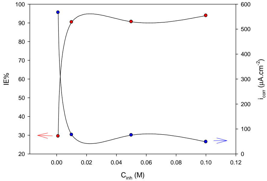
Fig.10: Variation of IE% and i_{corr} of A383 in 0.5 M H 3 PO 4 without and with different concentrations of K 2 CrO 4 .
