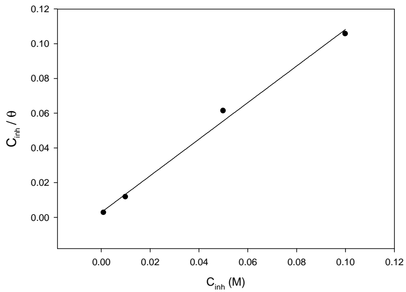
Fig.11:Langmuir isotherm adsorption mode of A383 at different concentration of K_2CrO_4 in 0.5 M H_3PO_4 solutions.
