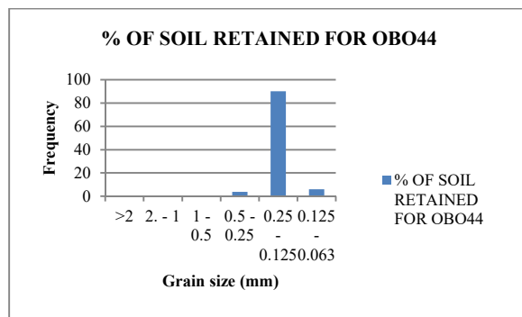
Figure 39: Histogram for sample OBO44
