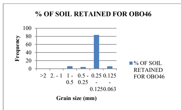
Figure 41: Histogram for sample OBO46
