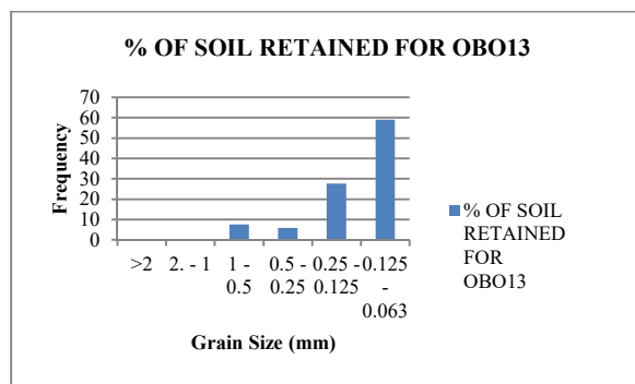
Figure 16: Histogram for sample OBO13
