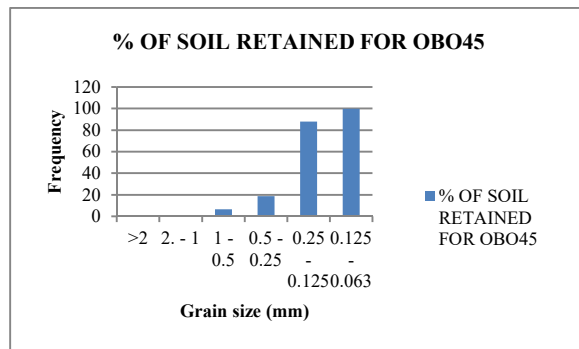
Figure 40: Histogram for sample OBO45
