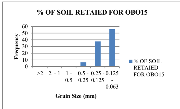
Figure 18: Histogram for sample OBO15
