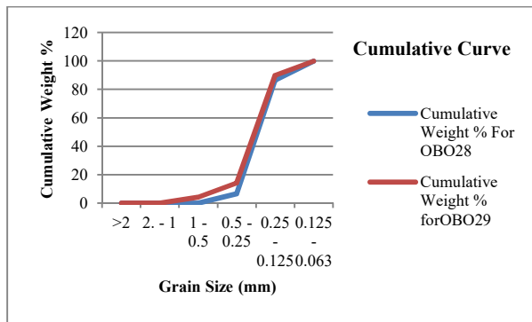
Figure 23: Cumulative curves for samples OBO28, and OBO29
