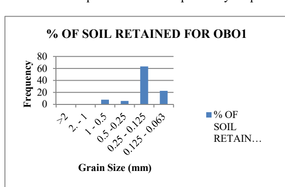
Figure 3: Histogram for sample OBO1
