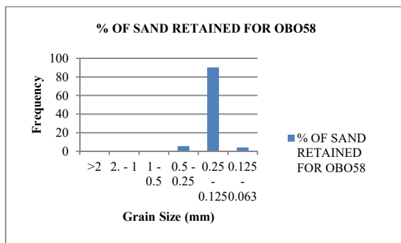
Figure 49: Histogram for sample OBO58
