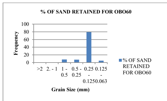
Figure 51: Histogram for sample OBO60
