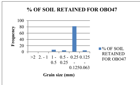
Figure 42: Histogram for sample OBO47
