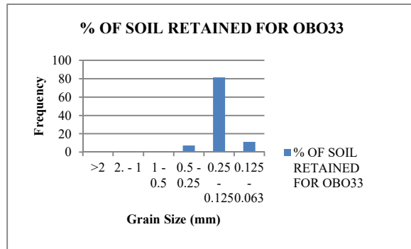
Figure 34: Histogram for sample OBO33
