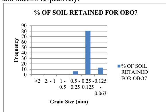
Figure 6: Histogram for sample OBO7
