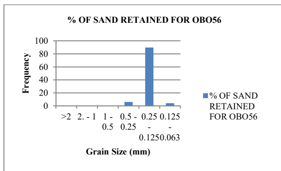
Figure 47: Histogram for sample OBO56
