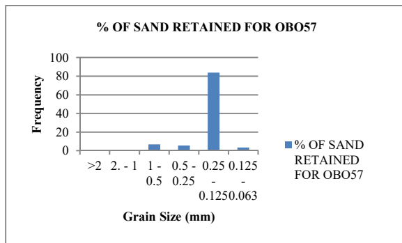
Figure 48: Histogram for sample OBO57
