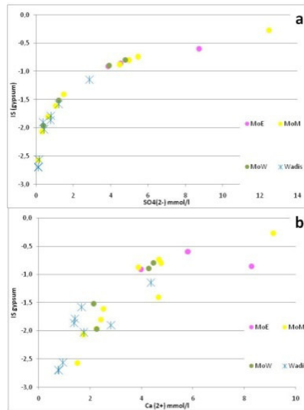
Figure .10 Scatter plot of saturation index of gypsum vs SO 4 (a) and Ca (b)
