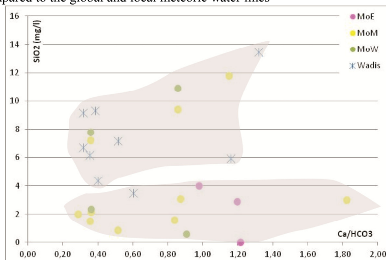
Figure .5 Scatter plot of \text{Ca}/\text{HCO}_3 vs \text{SiO}_2
