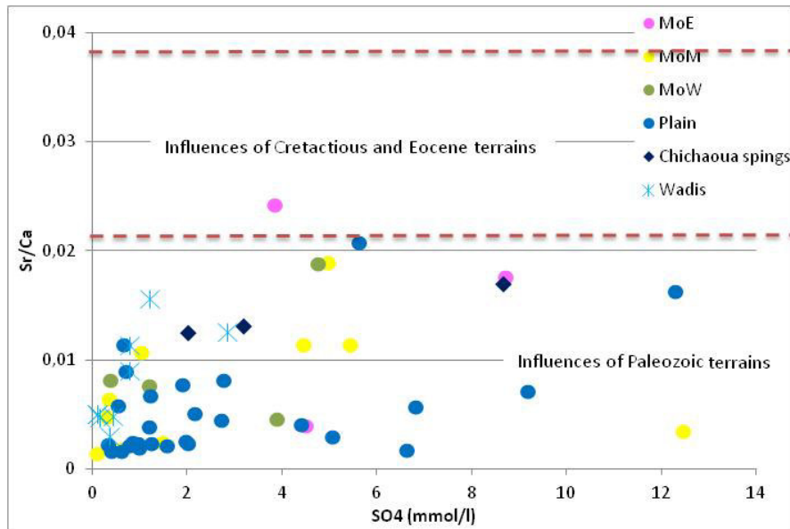
Figure .14 Variation of SO 4 concentration with Sr/Ca
