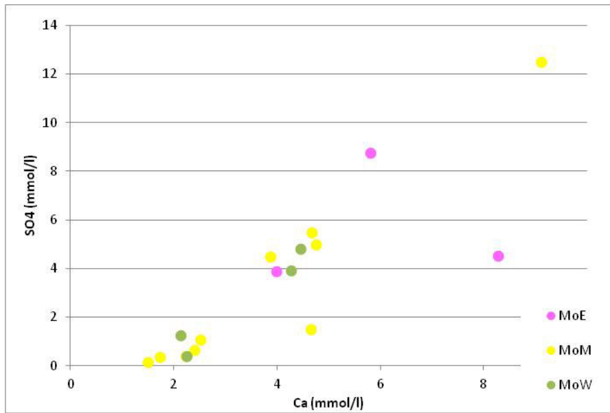
Figure .8 Scatter plot of Ca vs SO4
