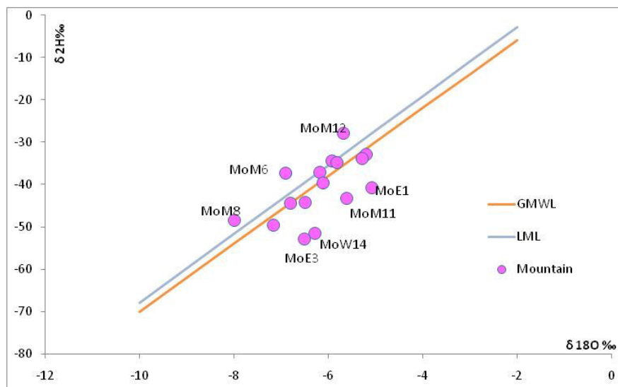
Figure .4 \delta^2\text{H} vs \delta^{18}\text{O} values of sampled, springs and surface waters of mountainous as compared to the global and local meteoric water lines
