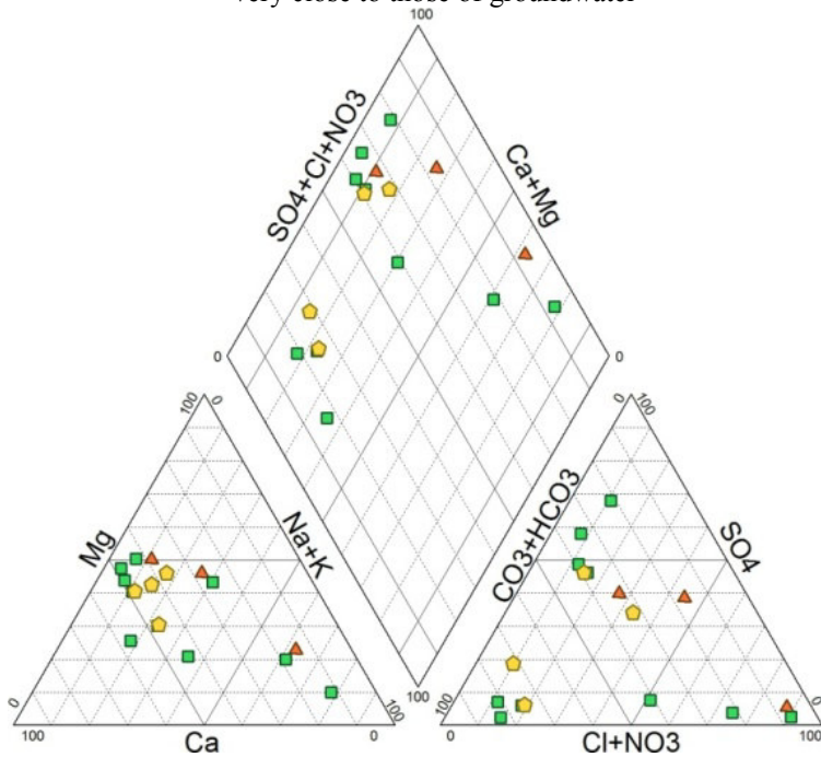
Figure .7 Piper diagram of the chemical composition of sampled groundwater
