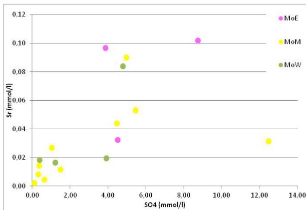
Figure .11 Scatter plot of Sr vs SO 4
