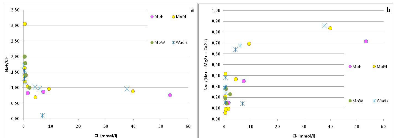
Figure .13 Variation of Cl concentration with Na/Cl ratio (a) and Na/(Na + Ca +Mg) ratio (b) in groundwaters of the piedmont area of High-Atlas mountain
