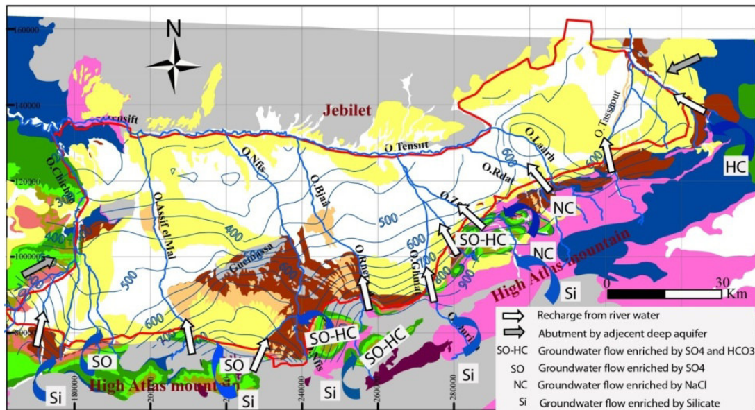
Figure .15 Mode of recharge and mineralization of groundwater in piedmont area of High-Atlas mountain and their adjacent Haouz plain.
