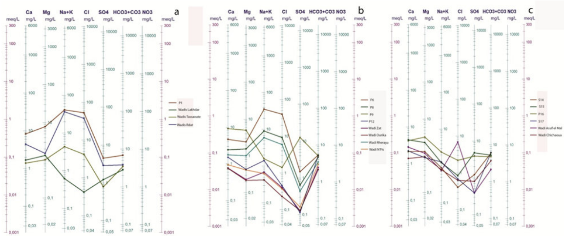
Figure .6 Fingerprint plot of chemical compositions of water samples. The chemical composition of river water very close to those of groundwater
