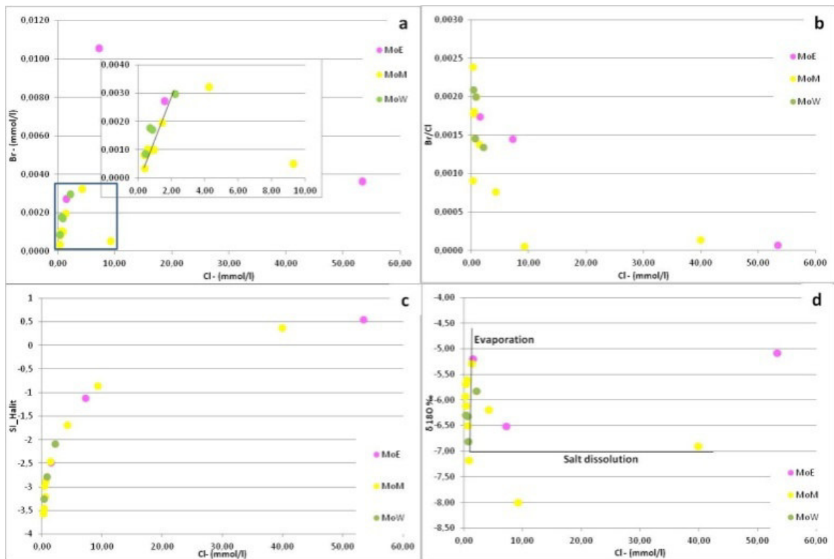
Figure .9 a) Scatter plot of Br vs Cl; b) Scatter plot Br/Cl vs Cl; c) Scatter plot of saturation index vs Cl and d) Scatter plot of 18O vs Cl concentrations in the study area
