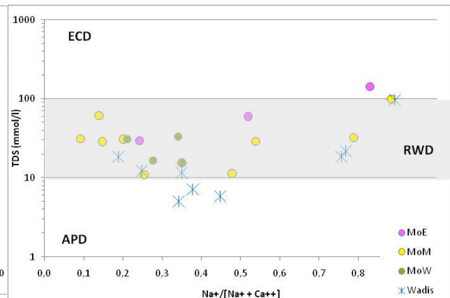
Figure .12 Gibbs diagram of groundwater samples in the piedmont area of High-Atlas
