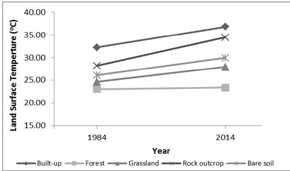
Figure 6: Land Surface Temperature (°C) over the different land use land covers in 1984 and 2014 for Akure
