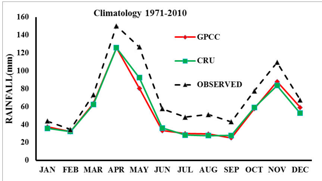
Fig. 2 Mean monthly for rainfall (RF CLIM) based on CRU, STN and GPCC, Kenya (longitude 34° E - 42° E and latitude 5° S - 5° N), 1971 -2010.
