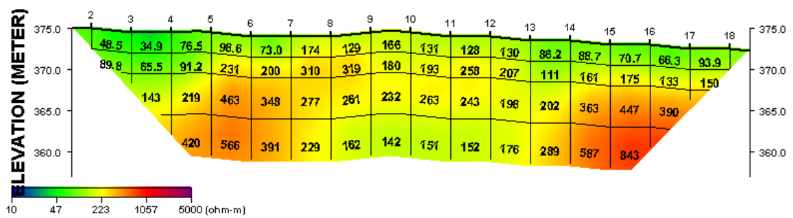
Figure 4. Dipole - dipole Pseudosection and VLE-EM Profile across the polluted area after two weeks
