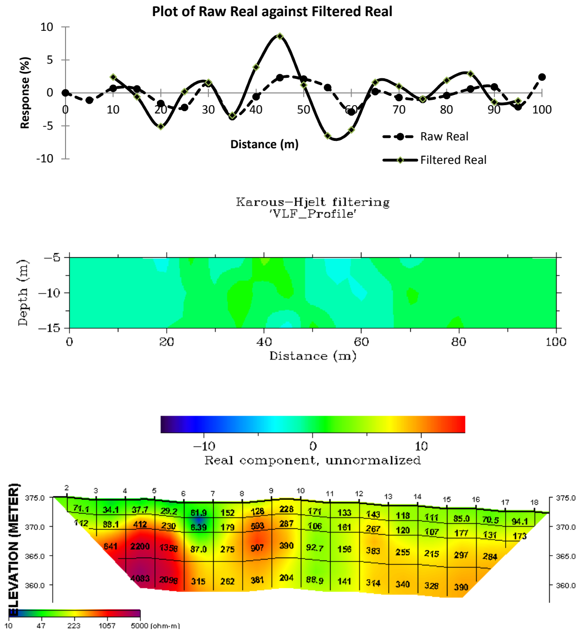
Figure 5. Dipole - dipole Pseudo-section and VLE-EM Profile across the polluted area after six weeks
