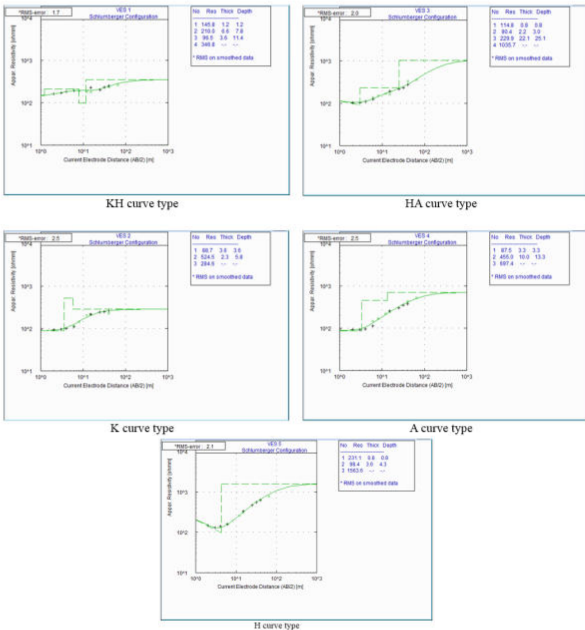
Figure 8. Iterated curves types obtained from the study area
