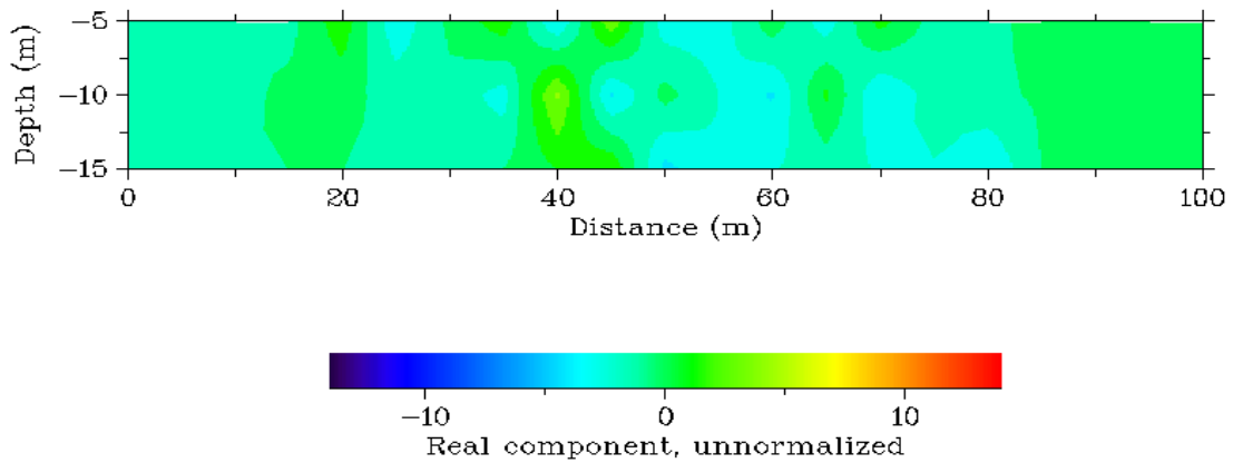
Figure 4. Dipole - dipole Pseudosection and VLE-EM Profile across the polluted area after two weeks
