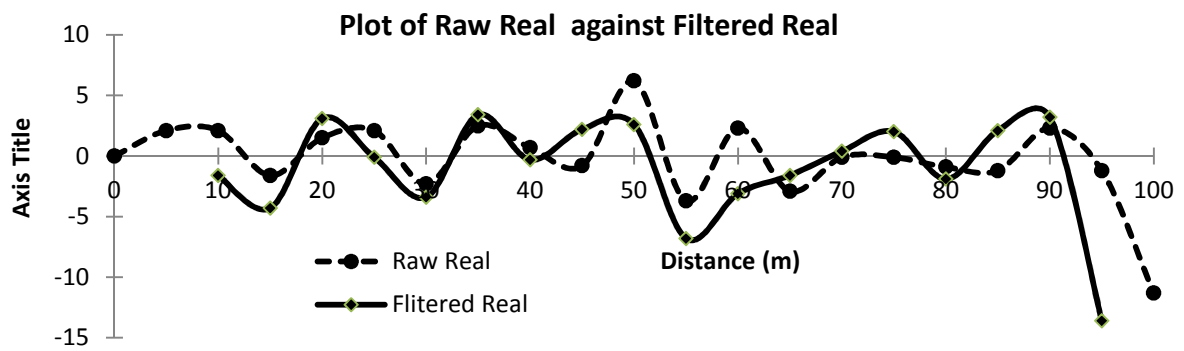
Karous-Hjelt filtering 'Synthetic' 'VLF' 'data'
