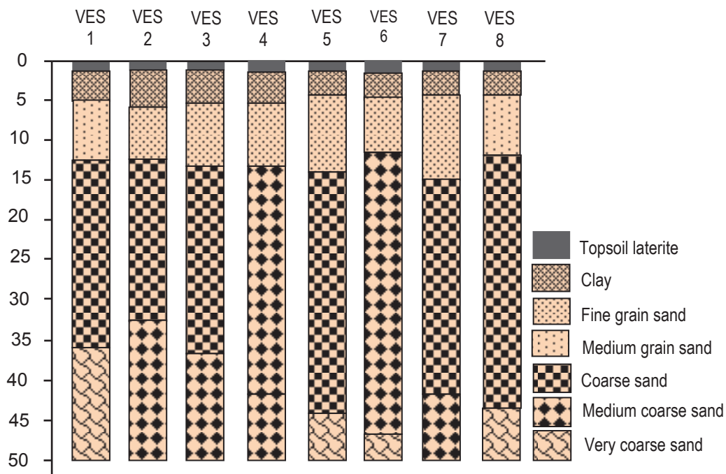
Fig. 6: Geoelectric profile of the survey area showing a five layer model
