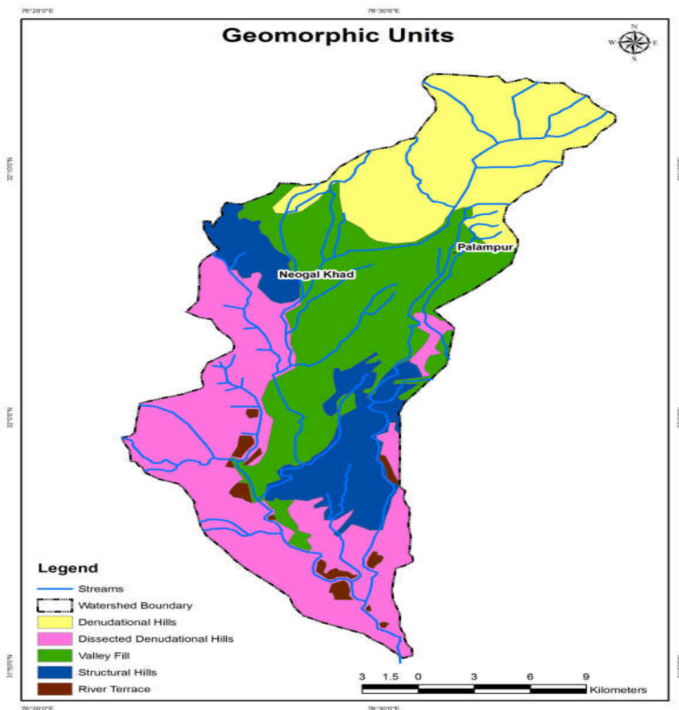
Figure 3: Different Geomorphic Units of the Neugal Watershed
