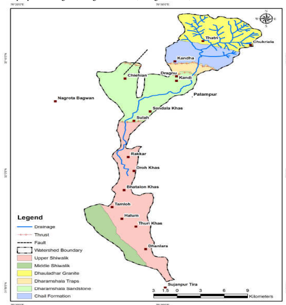
Figure 2. Geological Setting of Neugal Khad Watershed in District Kangra, Himachal Pradesh Geomorphological Analysis
