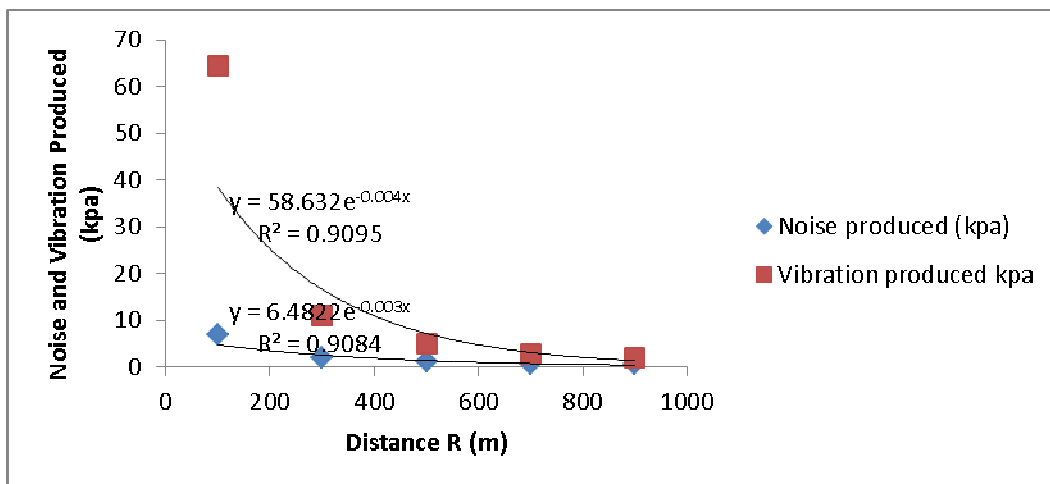
Fig. 12: Noise and Vibration produced against Distance using NONEL
