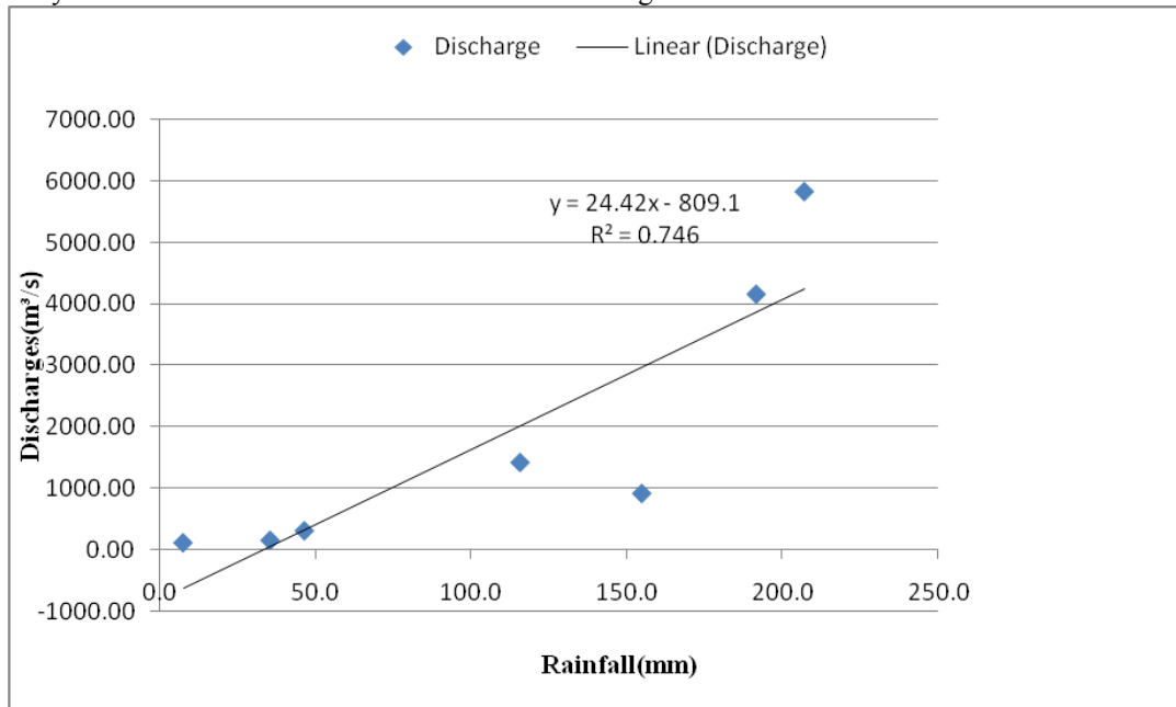
Figure 7. Cumulated Rainfall and Discharge relationship of 2008 of the White Volta River at Pwalugu
