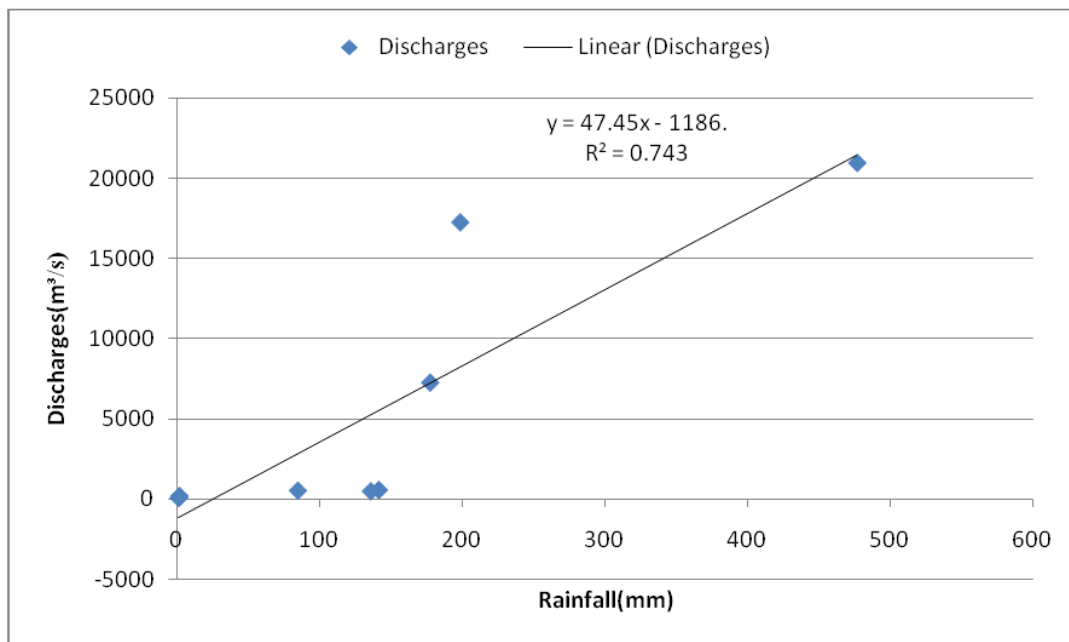
Figure 6, Cumulated Rainfall and Discharge relationship of 2007 of the White Volta River at Pwalugu
