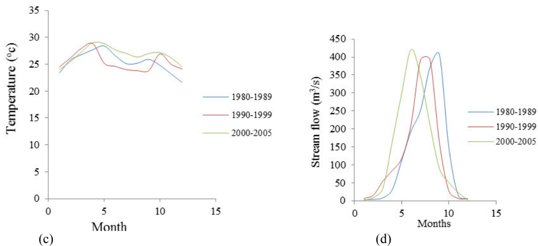
Figure 1: Decadal Segmentation of the Monthly hydro-meteorological variables: (a) Rainfall (b) Evaporation (c) Temperature and (d) Streamflow
