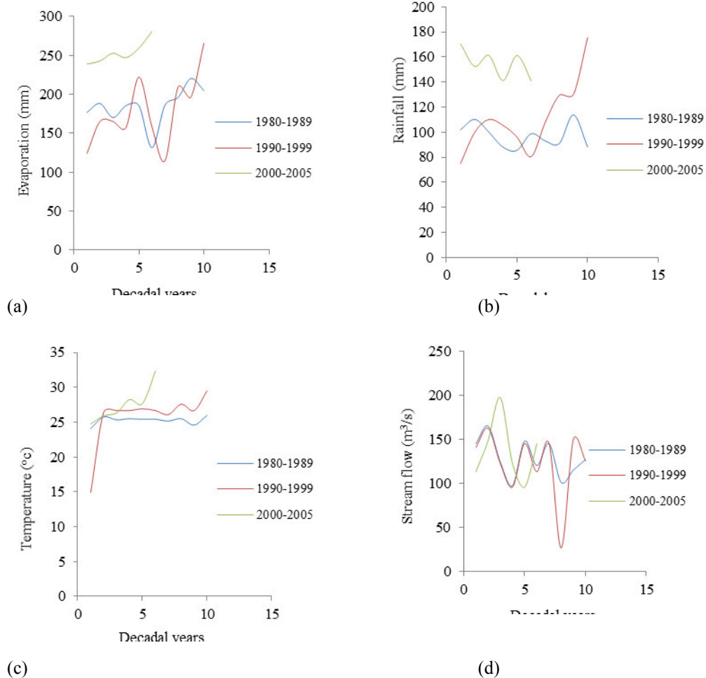
Figure 2: Decadal Segmentation of the Annual Hydro-meteorological variables (a) Rainfall (b) Evaporation (c) Temperature and (d) Streamflow
