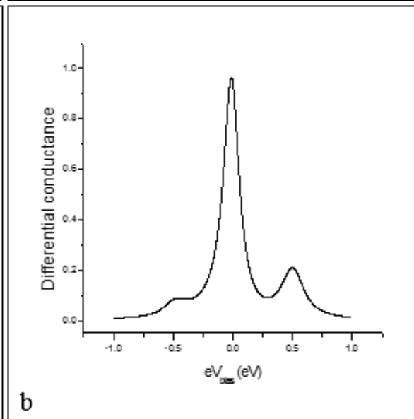
Fig. (11) showing (a) tunneling current as a function of bias voltage, (b) differential conductance as a function of bias voltage, when J = -0.4 eV U_1 = U_2 = 0.04 eV , \Gamma_{ia}^{\pm\sigma} = 0.08 eV E_1 = E_2 = 0.05 eV , V_{12} = 0.2 eV .
