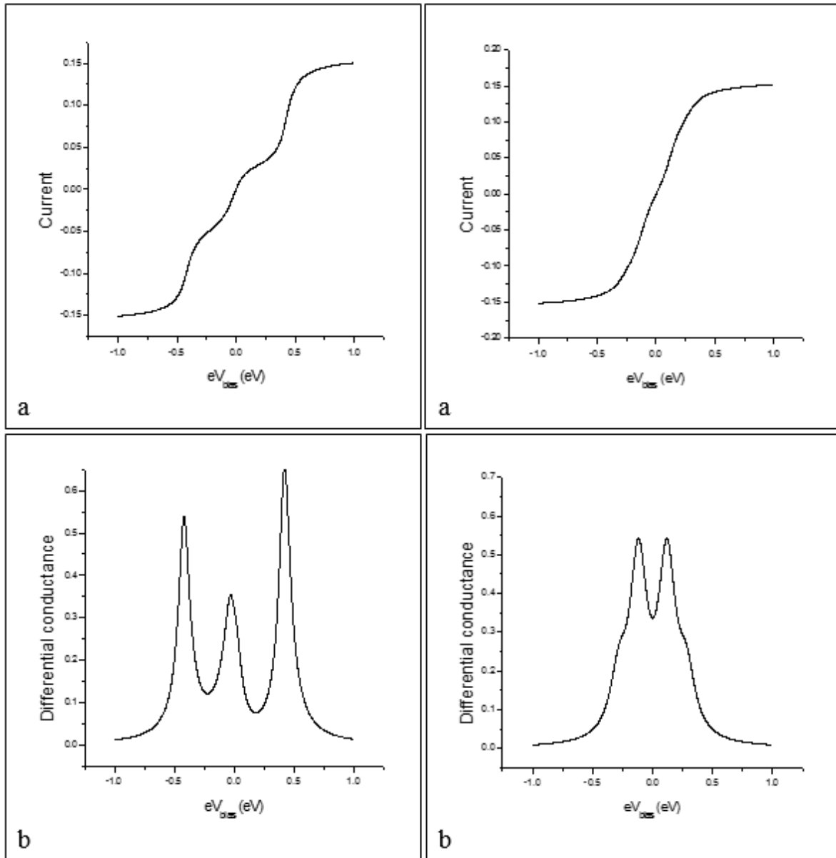
Fig. (6) showing (a) tunneling current as a function of bias voltage, (b) differential conductance as a function of bias voltage, when J = 0.4 eV U_1 = U_2 = 0.04 eV , \Gamma_{ia}^{\pm\sigma} = 0.08 eV E_1 = E_2 = 0.05 eV , V_{12} = 0.2 eV .
