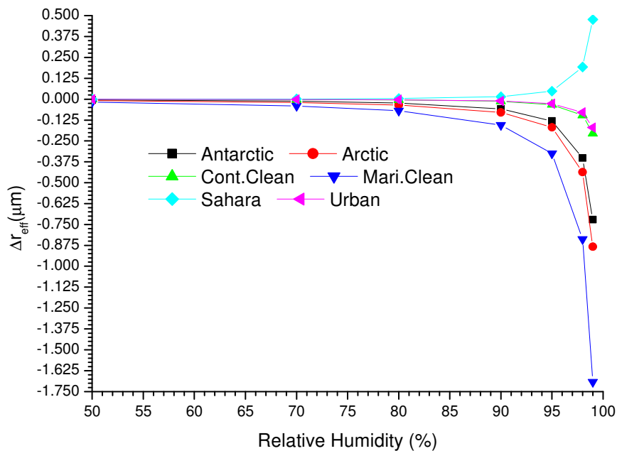
Figure 12 A plot of \Delta r_{eff}(RH) of the aerosols against Relative Humidity using equation (24).
