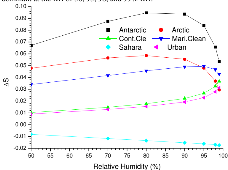
Figure 4: A plot of \Delta S of the aerosols against Relative Humidity using equation (14).
