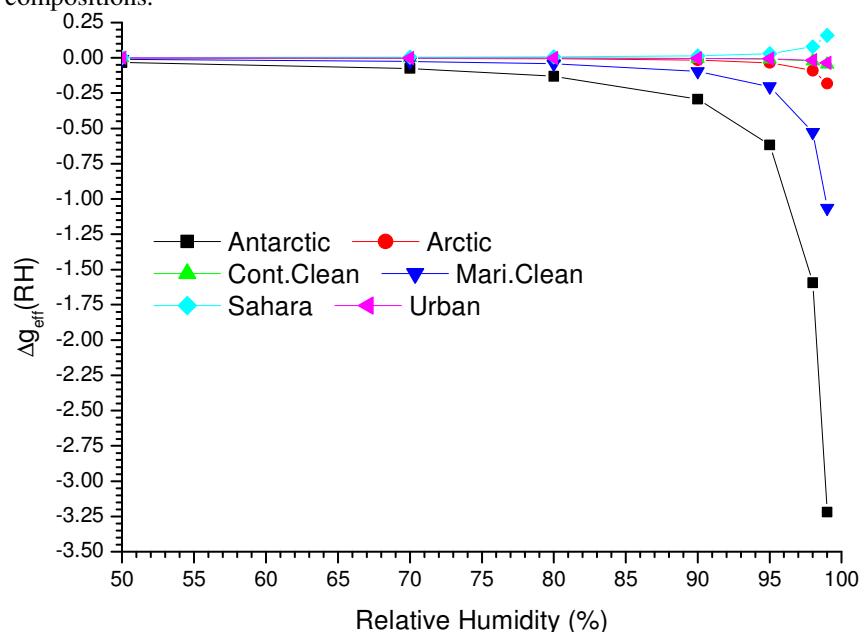
Figure 7: A plot of \Delta g_{eff}(RH) of the aerosols against Relative Humidity using equation (18)
