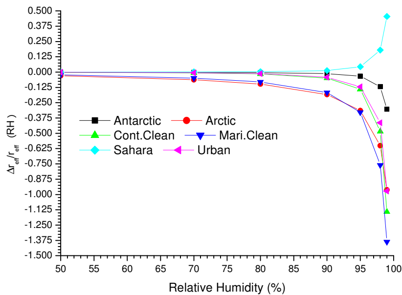
Figure14: A plot of \Delta r_{eff}/r_{eff}(RH) of the aerosols against Relative Humidity using equation (26).
