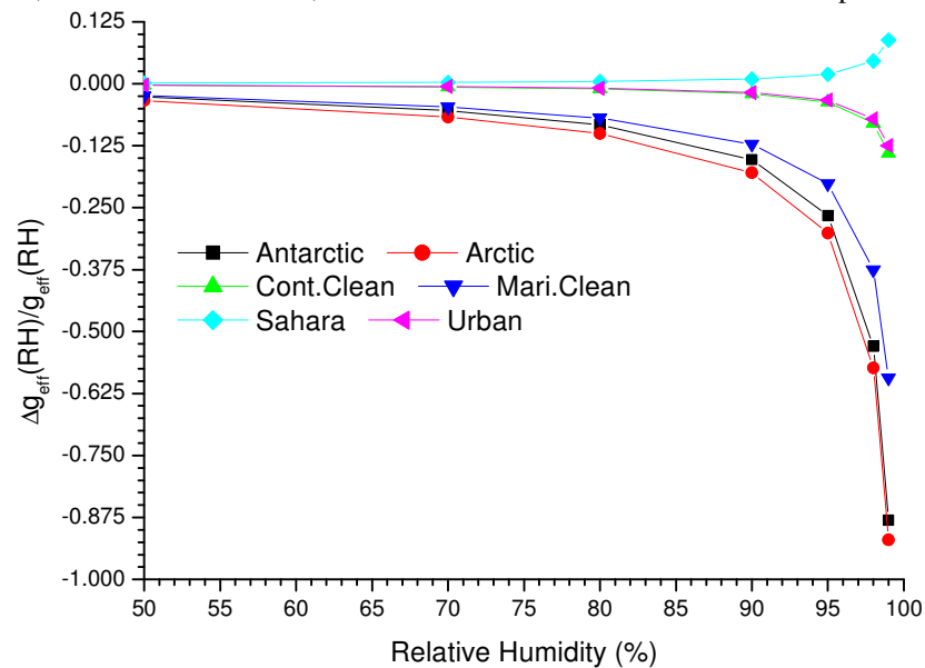
Figure 9: A plot of \Delta g_{eff}/g_{eff}(RH) of the aerosols against Relative Humidity using equation (20).
