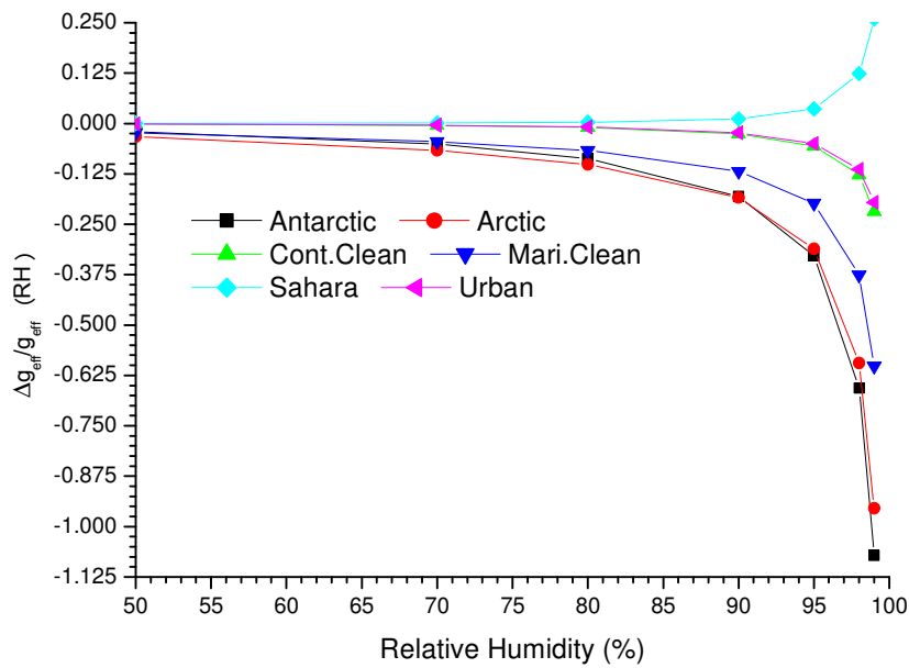
Figure13: A plot of \Delta g_{eff}/g_{eff}(RH) of the aerosols against Relative Humidity using equation (25).
