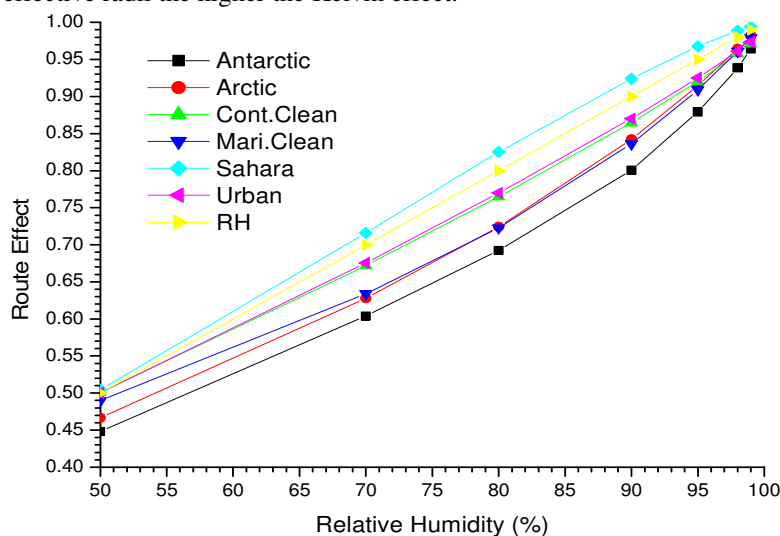
Figure 2: A plot of Route effect (water activity) of the aerosols against Relative Humidity using equation (12b).
