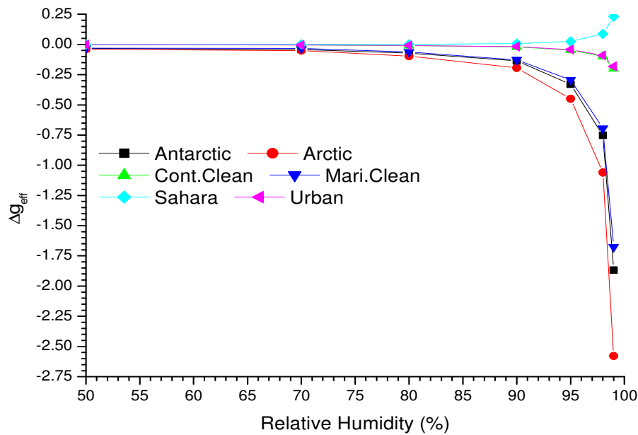
Figure 5: A plot of \Delta g_{eff} of the aerosols against Relative Humidity using equation (15).
