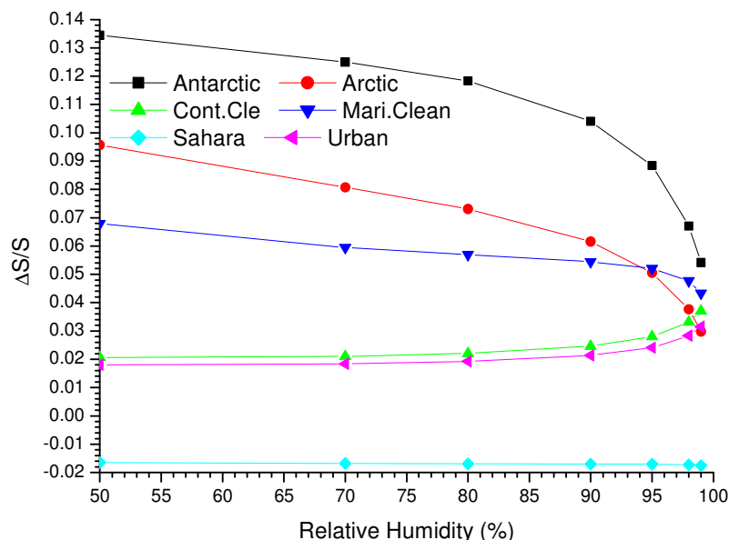
Figure 15: A plot of \Delta S/S of the aerosols against Relative Humidity using equation (13) and the ambient RHs.
