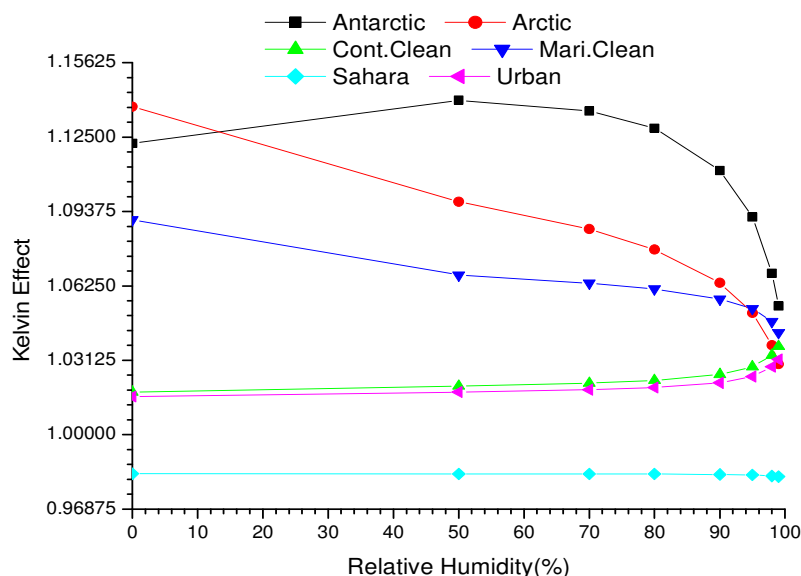
Figure 1: A plot of Kelvin effect of the aerosols against Relative Humidity using equation (11b).
