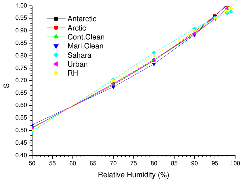
Figure 3: A plot of S(RH) of the aerosols against Relative Humidity using equation (13).
