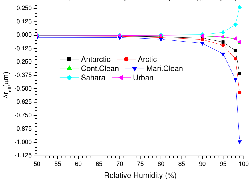
Figure 6: A plot of \Delta r_{eff} of the aerosols against Relative Humidity using equation (16).
