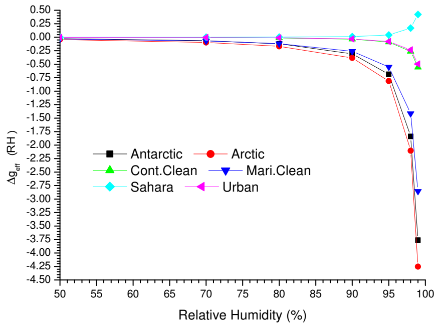
Figure 11: A plot of \Delta g_{eff}(RH) of the aerosols against Relative Humidity using equation (23).
