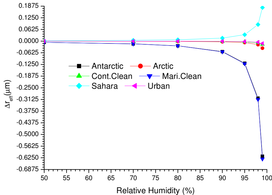
Figure 8 : A plot of \Delta r_{eff}(RH) of the aerosols against Relative Humidity using equation (19).
