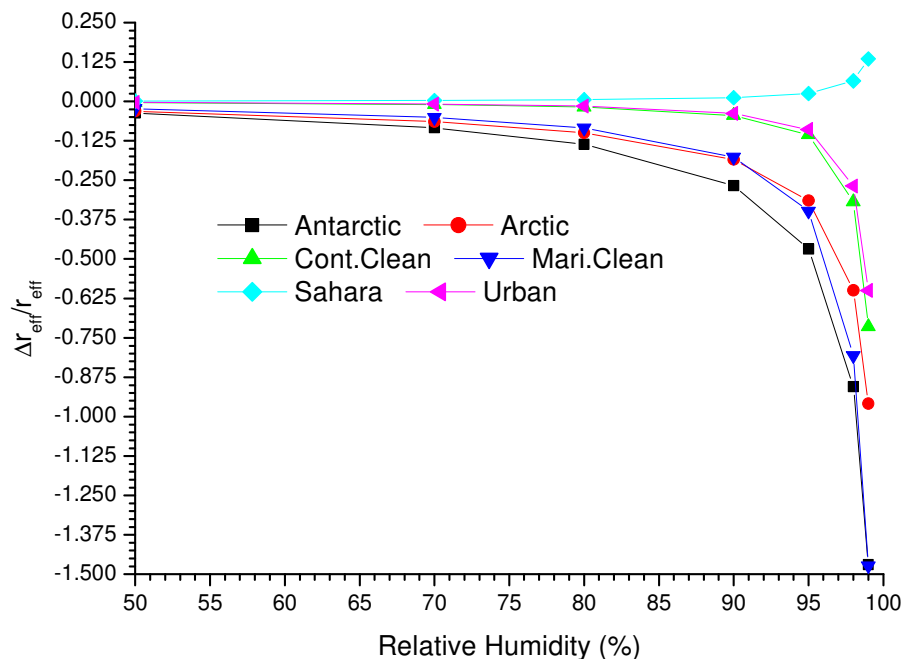
Figure 10: A plot of \Delta r_{eff}/r_{eff}(RH) of the aerosols against Relative Humidity using equation (21).
