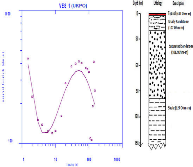
Fig 3a: Geoelectric curve and section at VES 1
