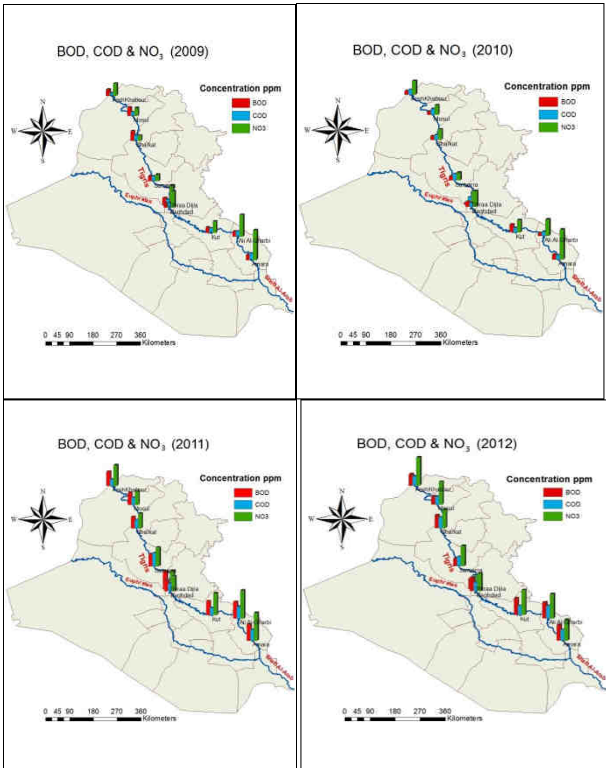
Fig.8 : Variations of NO 3 ,BOD and COD of the present stations for the study period.
