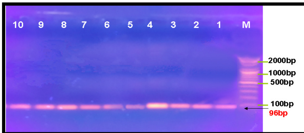
Figure (A: 2) gel electrophoresis that the results of the polymerase chain reaction to the boom raster point mutation of the gene ERG11-2-resistant anti-fungal using PCR RT-. Where M = DNA Ladder marker (100-2000bp), pathogenic isolates showed a positive result for gene ERG11-2 is responsible for increasing expression of gene to resistance to antibiotics KT, FLC, CC. Sample (6) for Candida tropicalis , samples (1-5,8,9) for C. albicans , the sample (10) for C. krusei and the sample (7) for C. parapsilosis .
