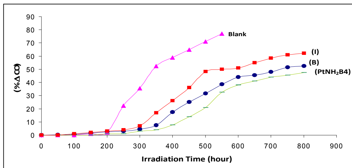
Fig (5) : change of transmittance intensity of carbonyl band against the time of U.V. irradiation
