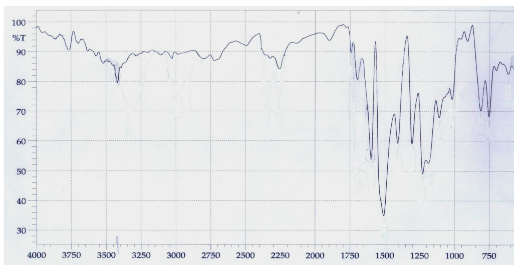
Fig(4) : IR spectrum of \text{NiNH}_2\text{B}_4
