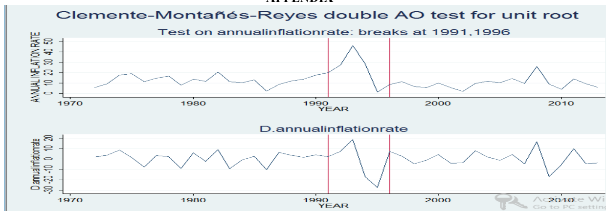
Figure A1.1: Clemente-Montañés -Reyes AO Test, Inflation.
