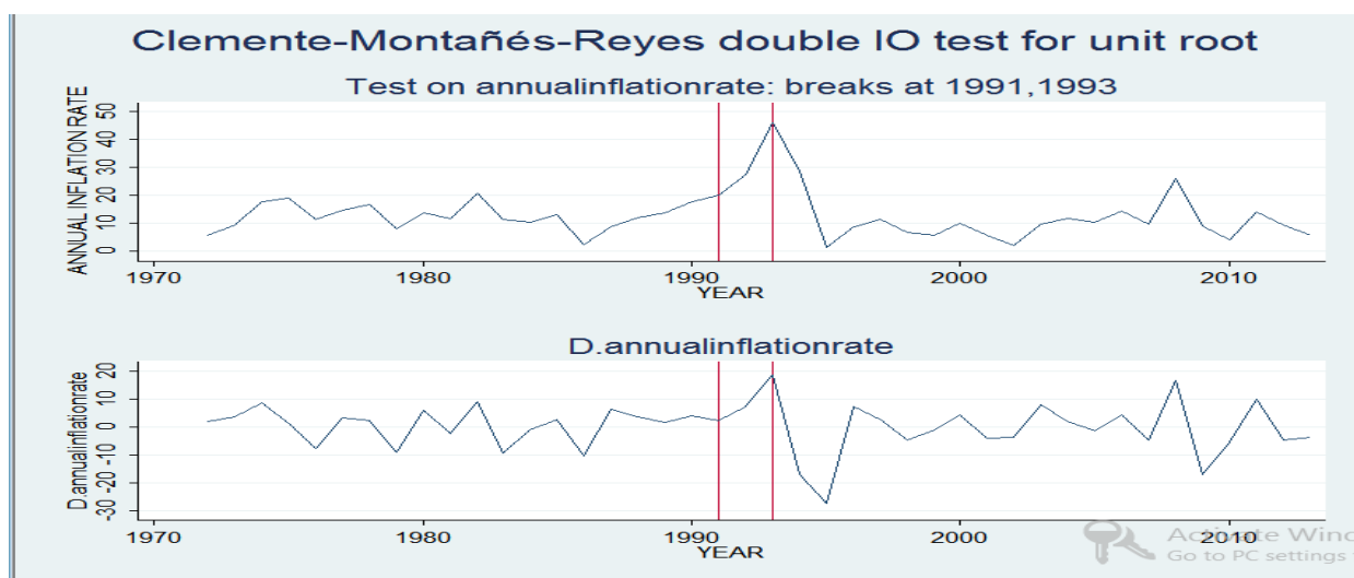
Figure A1.2: Clemente-Montañés -Reyes IO Test, Inflation
