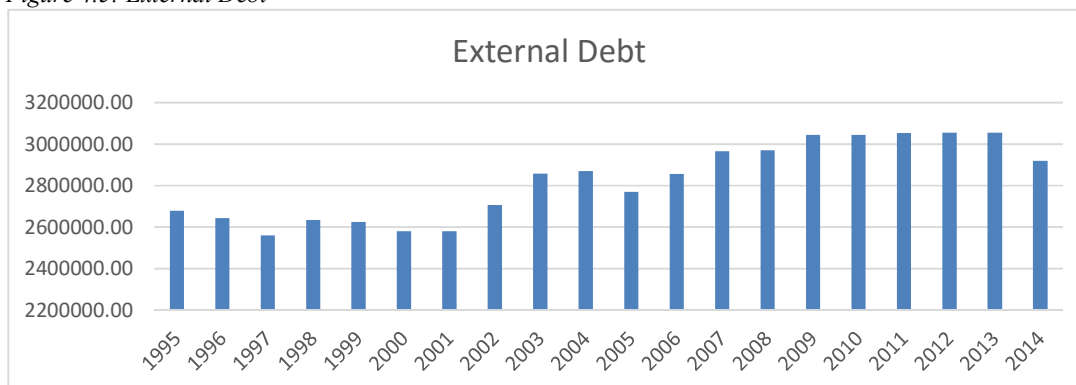
Figure 4.5: External Debt
