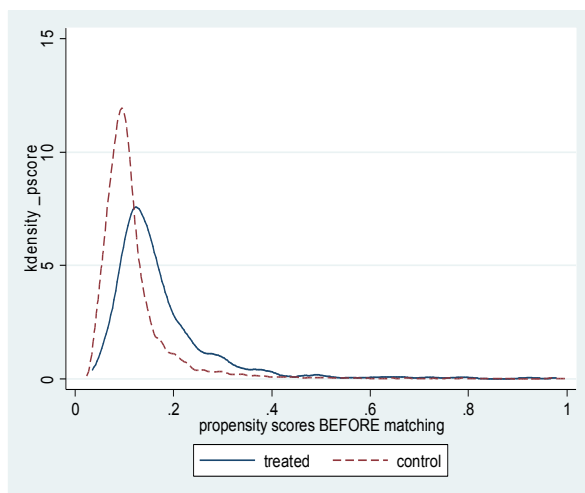
Figure 2: PSM kernel density before matching
