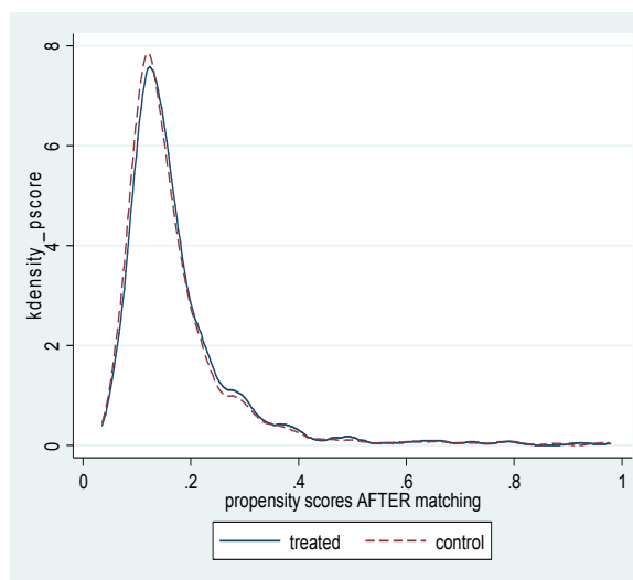
Figure3: PSM kernel density after matching
