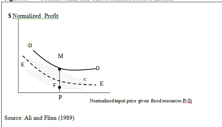
Figure 2: Frontier MLE and OLS Stochastic Profit Function
