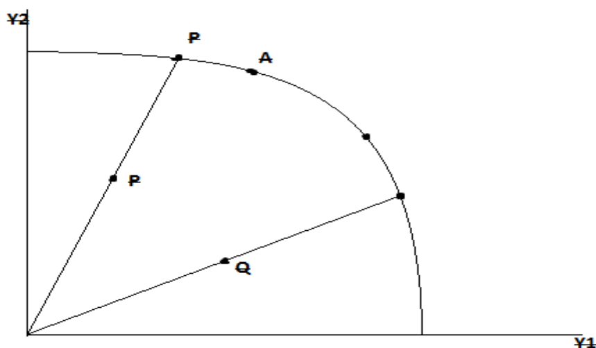
Figure 2: Output Oriented DEA.
