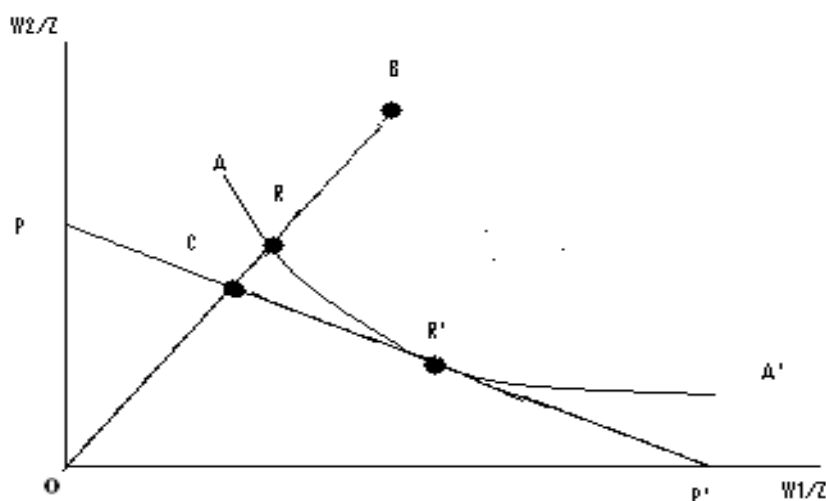
Figure 1: Input Oriented Technical Efficiency.
