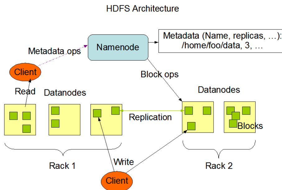
Figure 3.3.1 HDFS ARCHITECTURE [14]
