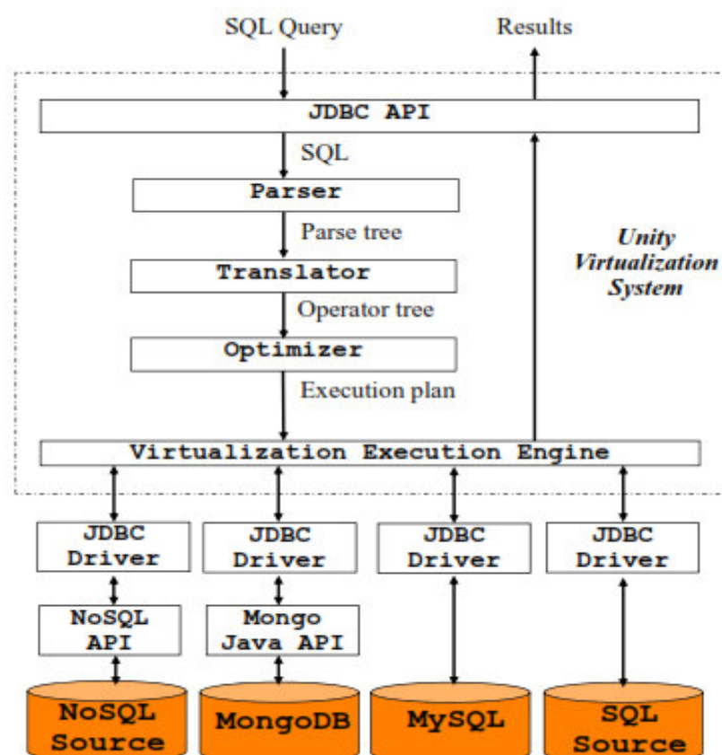
Figure 2.2 Unity Architecture
