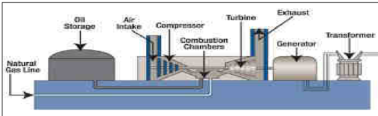
Figure (1) gas turbine power plant
