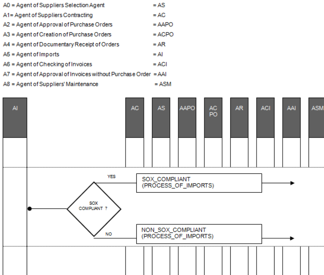
Fig. 5. Joint Deliberative Dialog Protocol (Inquire).
