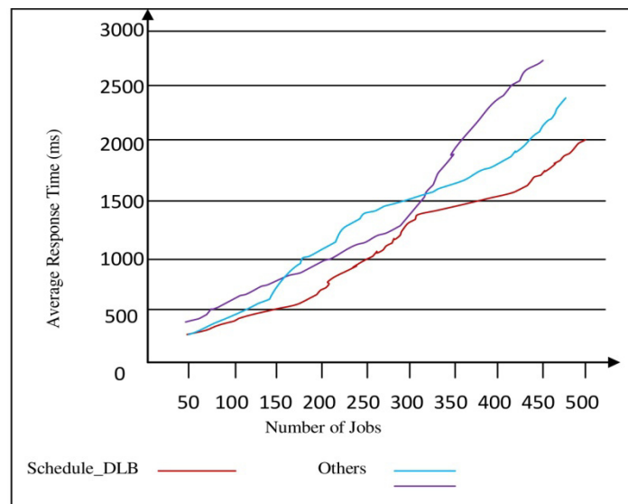
Figure4: Analysis with other load balancing algorithm
