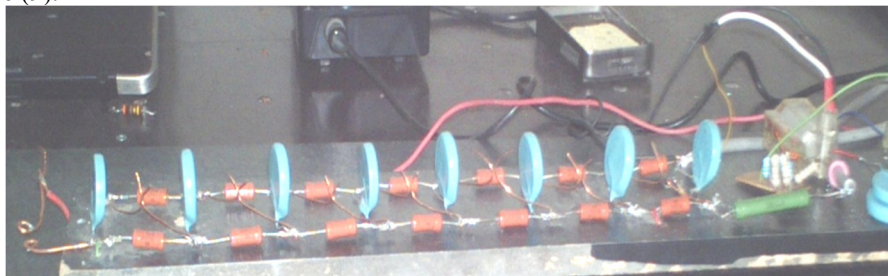
Fig. (9) Marx generator (8-stage).
