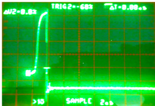
Figure (14) Voltage pulse for Marx generator- third stage 4.5kV.
