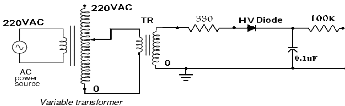
Fig. (5) A homemade high voltage power supply.
