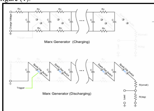
Fig. (1) Marx Generator (A) Charging (B) Discharging [Kuffel E. and Abdullah M.].
