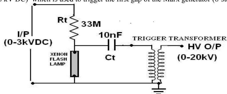
Fig. (6) Xenon flash lamp trigger circuit
