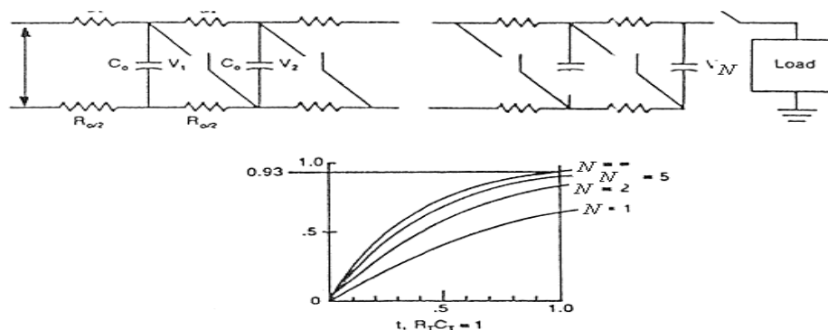
Fig. (3) Marx bank charging performance [Sarjeant W. J. and Dollinger R. E.].
