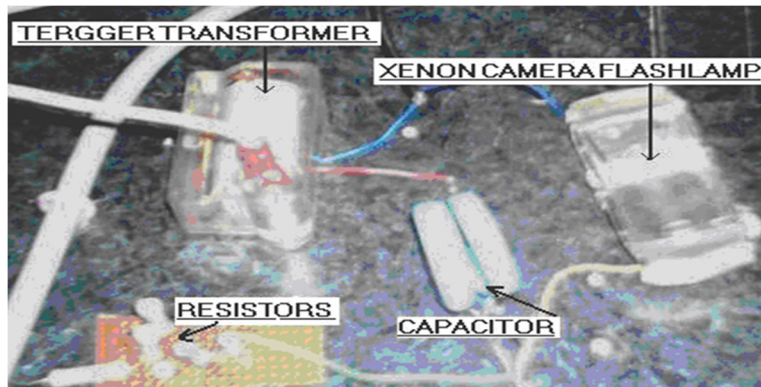
Fig. (7) Camera flash lamp triggers circuit.
