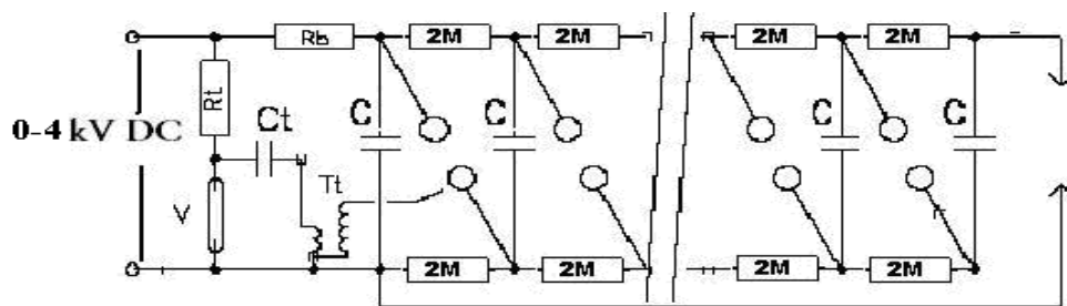
Fig. (8) Circuit diagram for Marx generator (8-stage).
