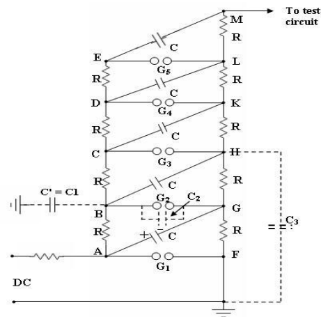
Fig. (2) Basic circuit of a five-stage impulse generator [ Kuffel E. and Abdullah M.].
