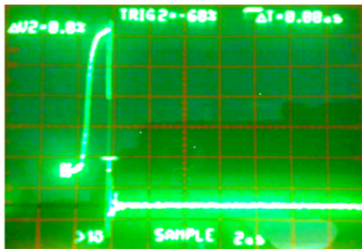
(a) Full voltage pulse, scale (1V, 2μs)
