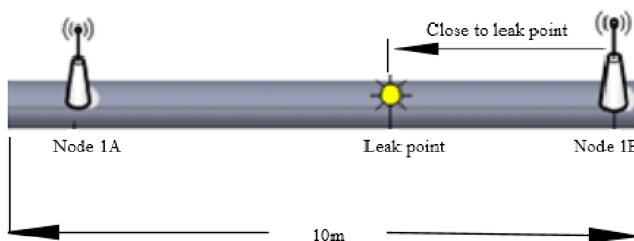
Figure 1. Acoustic wireless sensor node on pipeline network architecture
