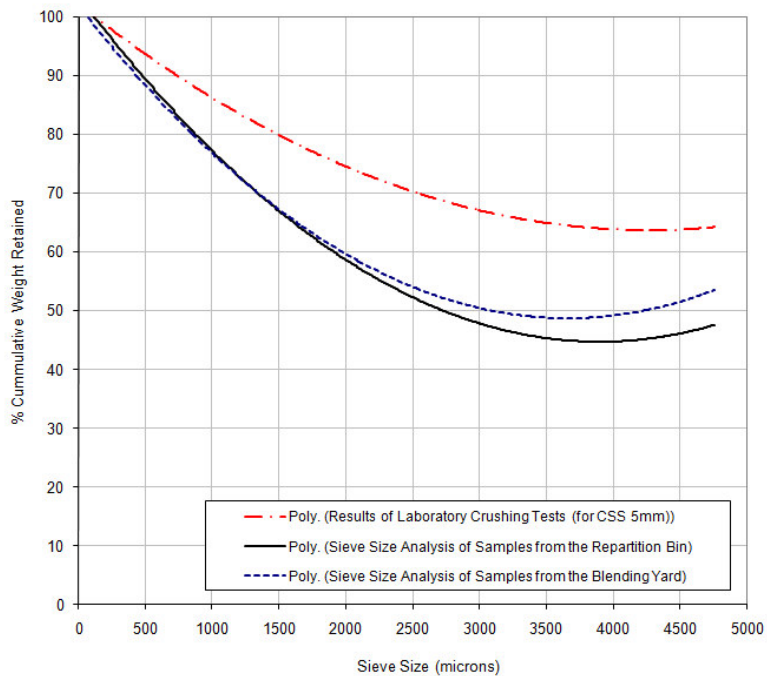
Figure 8: Comparison of Size Distribution of Material in the Blending Yard and Repartition Bin with Crushing Tests
