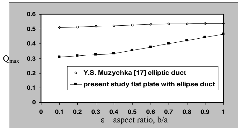
Fig. 17. comparison present study flat plate with ellipse duct with the results of Muzychka (2005)[17]
