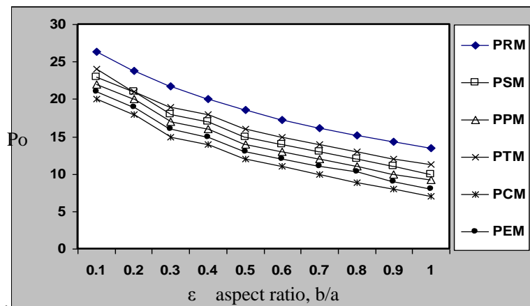
Fig. 9. Effect of channel aspect ratio on the Poiseuille numbers at Pr=10 and the number of passages equal to n=8 for all models.
