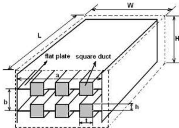
Fig. 1. Convectively cooled finite volume for the flat plate with square duct geometry micro channels
