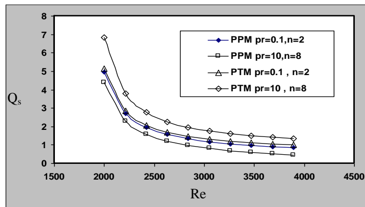
Fig.15. the relation between Reynolds number Re and the heat transfer rate ( Q_s ) for the models of rectangular and square passages shapes
