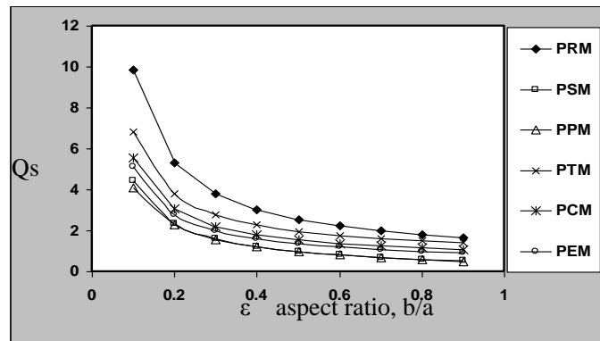
Fig. 12. Effect of channel aspect ratio on the heat transfer rate ( Q_s ) at Pr=0.1 and the number of passages equal to n=2 for all models.
