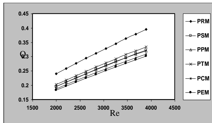
Fig. 4. Effect of Reynolds number Re on the efficient of heat dissipation at Pr=0.1 and the number of passages equal to n=2 for all models.
