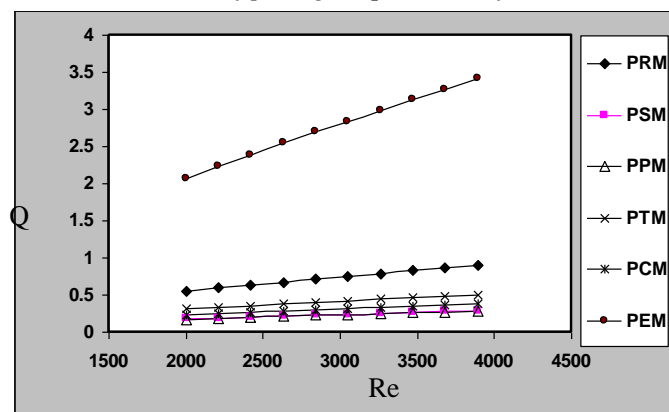
Fig.10. Effect of Reynolds number Re on the efficient of heat dissipation at Pr=10 and the number of passages equal to n=8 for all models.
