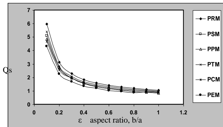
Fig. 7. Effect of channel aspect ratio on the heat transfer rate ( Q_s ) at Pr=0.1 and the number of passages equal to n=2 for all models.
