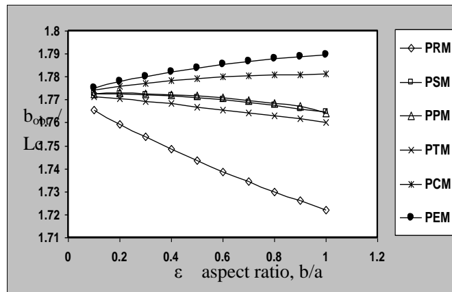
Fig. 5. Effect of channel aspect ratio on the optimal plate spacing ( b_{opt}/Lc ) at Pr=0.1 and the number of passages equal to n=2 for all models.
