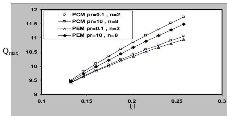
Fig.16. the relation between maximum heat transfer rate ( Q_{max} ) and the average velocity U for the models of rectangular and square passages shapes
