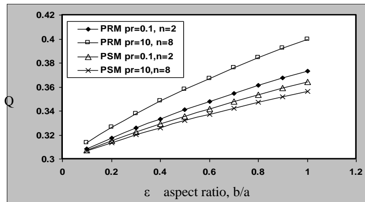
Fig.14. the relation between channel aspect ratio and the efficient of heat dissipation for the models of rectangular and square passages shapes
