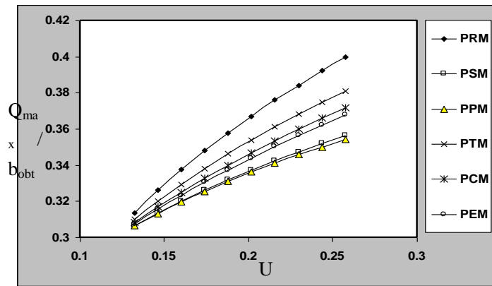
Fig. 11. Effect of average velocity on the optimal heat transfer plate spacing ( Q_{max} / b_{opt} ) at Pr=0.1 and the number of passages equal to n=2 for all models.
