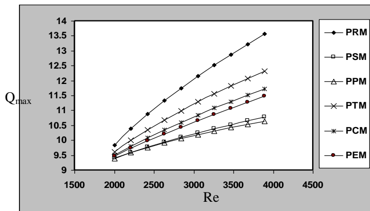
Fig. 13. Effect of channel aspect ratio on the maximum heat transfer rate ( Q_{max} ) at Pr=0.1 and the number of passages equal to n=2 for all models.
