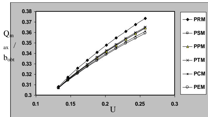
Fig. 6. Effect of average velocity on the optimal heat transfer plate spacing ( Q_{max}/b_{opt} ) at Pr=0.1 and the number of passages equal to n=2 for all models.
