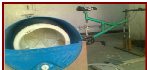
Fig.8 Pedal powered washing machine
