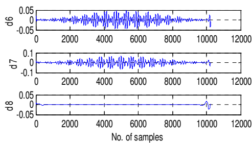
Fig. 9 Detail Co-efficient at 6 th ,7 th ,8 th level at single mass load ( faulty Condition, 10% turn short)
